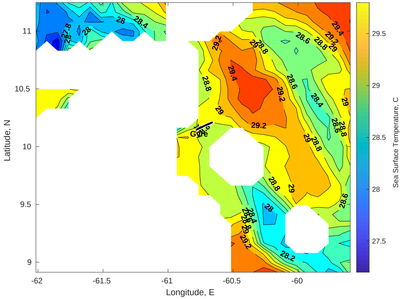
SST for Gyre at 27-Oct-2025 00:00:00
