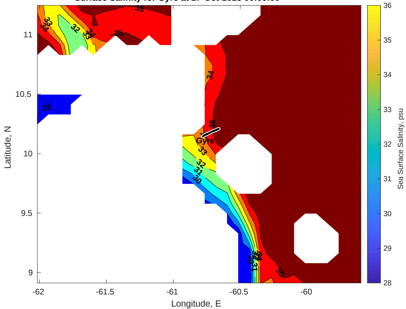
Surface Salinity for Gyre at 27-Oct-2025 00:00:00
