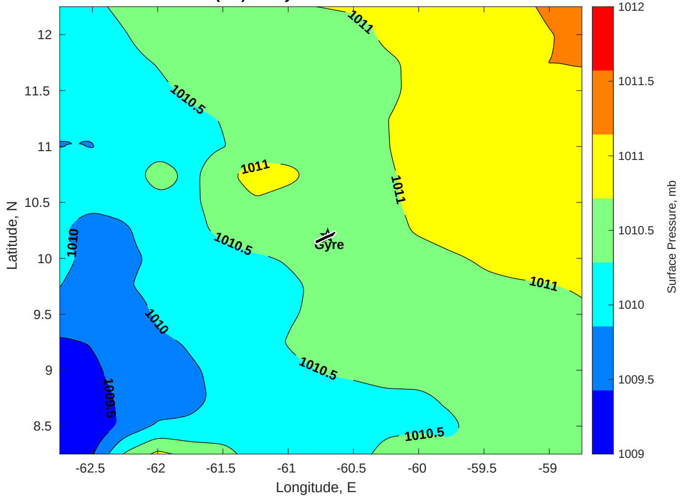
Surface Pressure (mb) for Gyre at 28-Oct-2025 00:00:00
