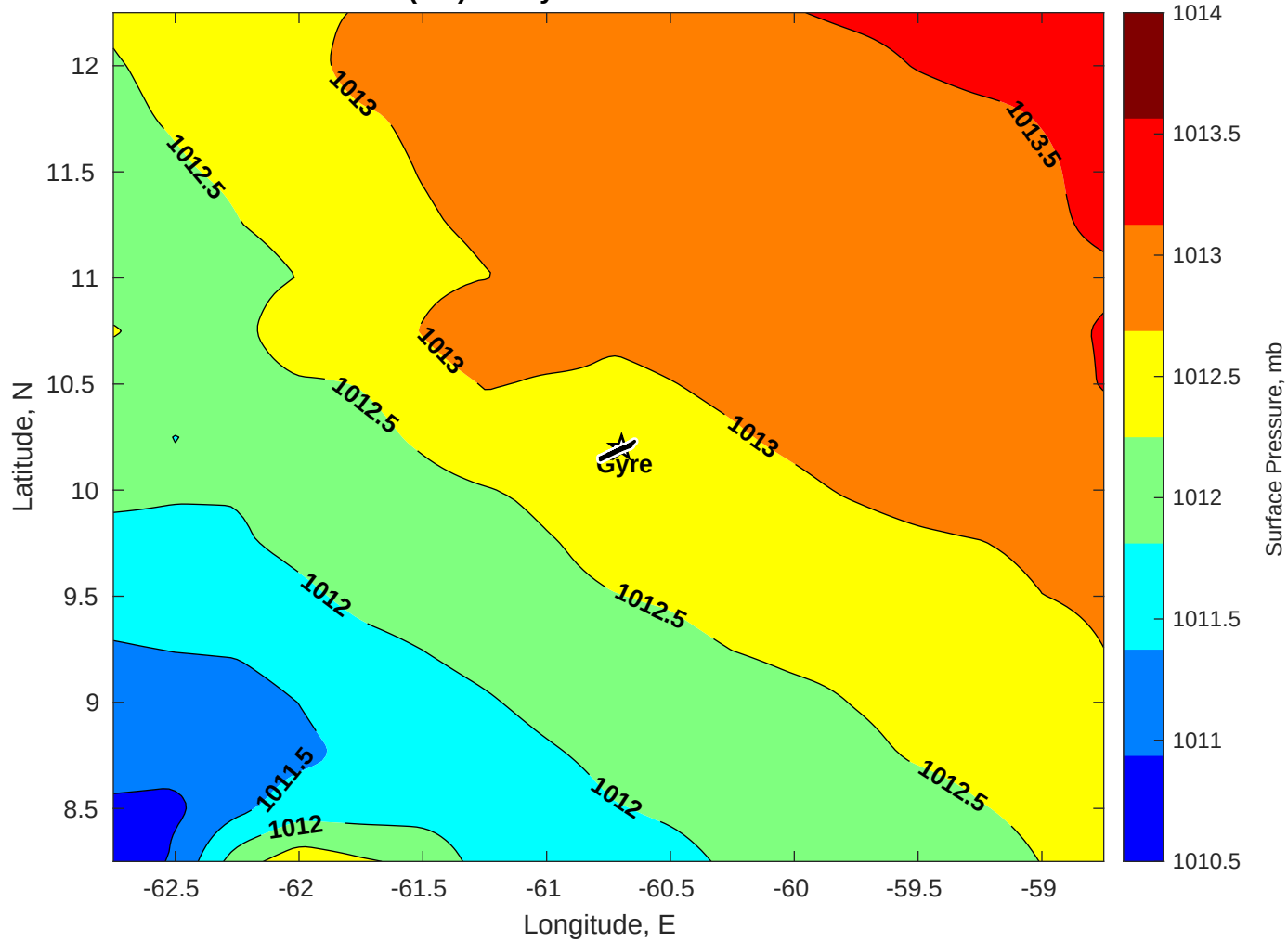
Surface Pressure (mb) for Gyre at 29-Oct-2025 00:00:00
