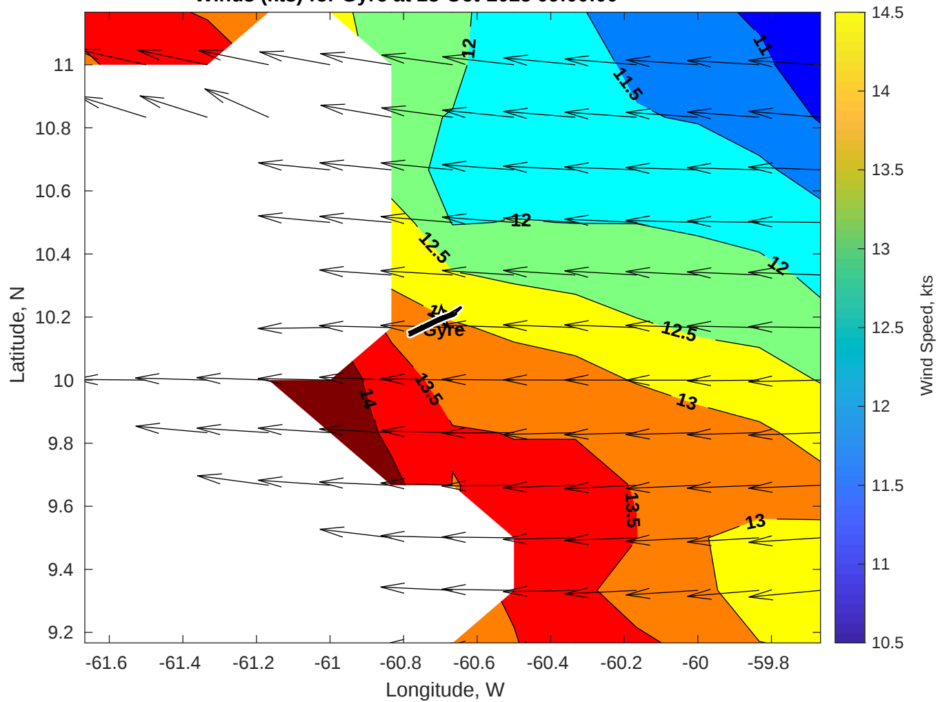
Winds (kts) for Gyre at 28-Oct-2025 09:00:00
