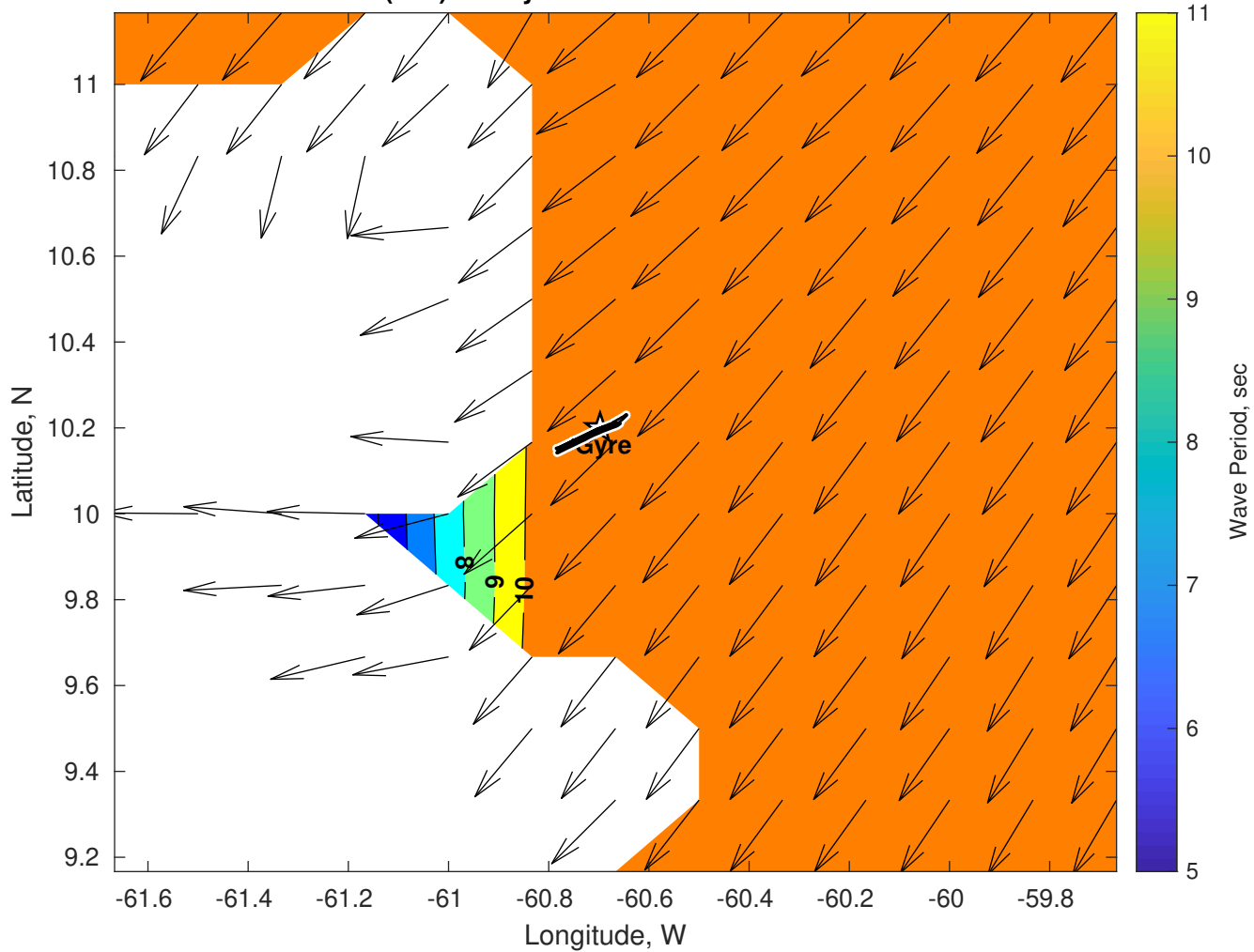
Wave Period (sec) for Gyre at 28-Oct-2025 09:00:00
