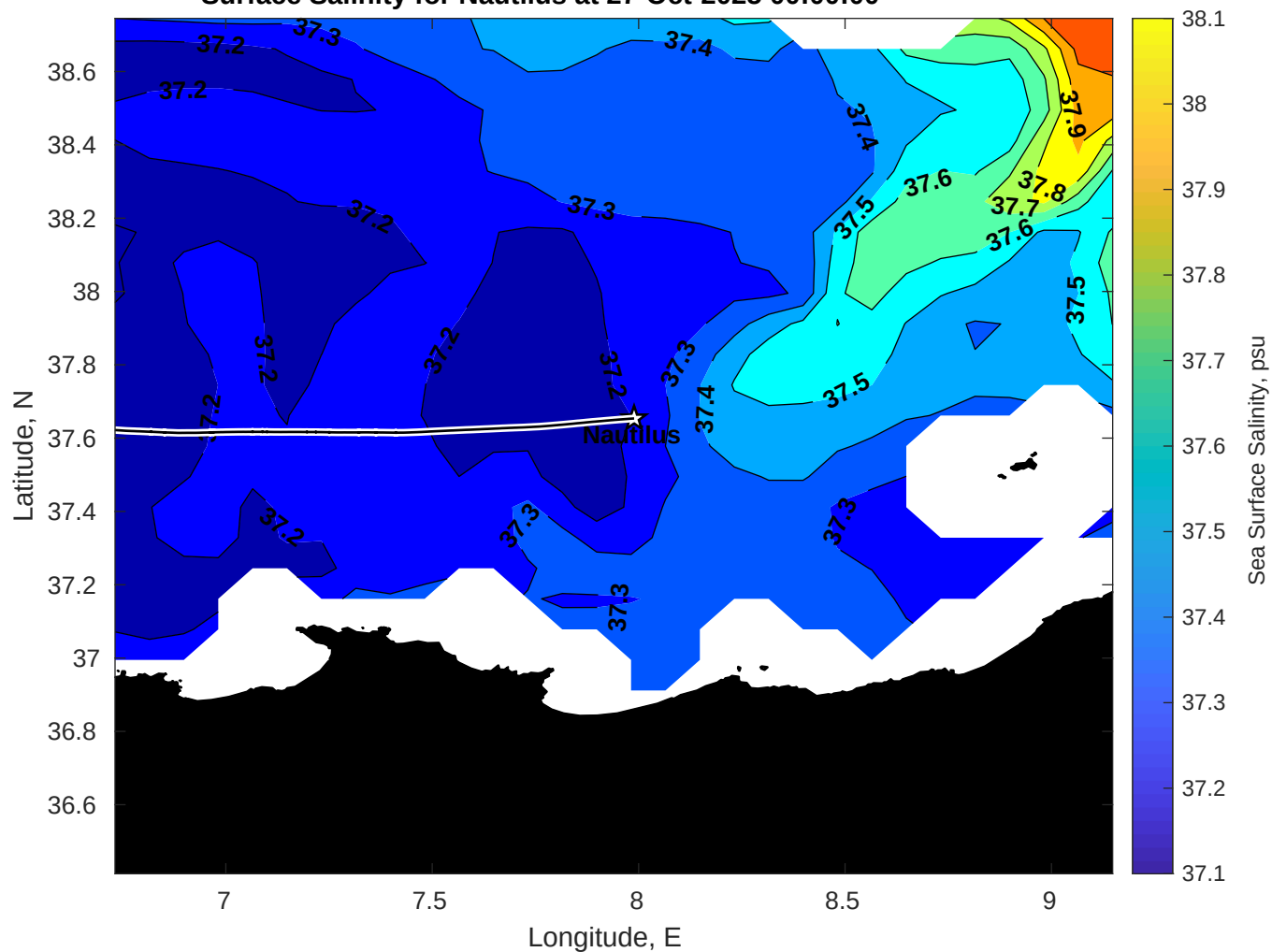
Surface Salinity for Nautilus at 27-Oct-2025 00:00:00
