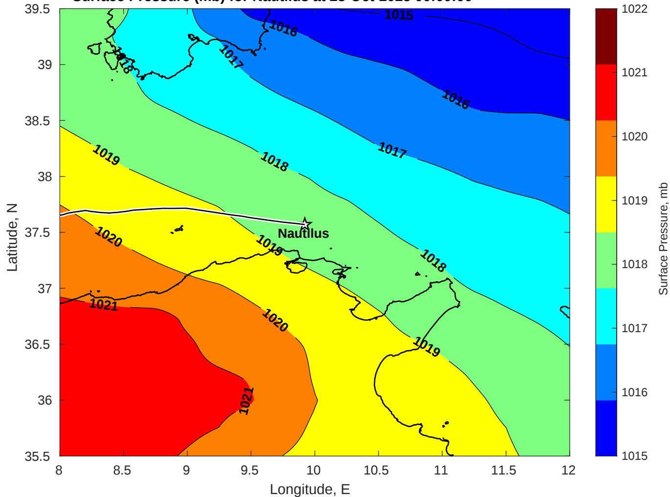
Surface Pressure (mb) for Nautilus at 28-Oct-2025 00:00:00
