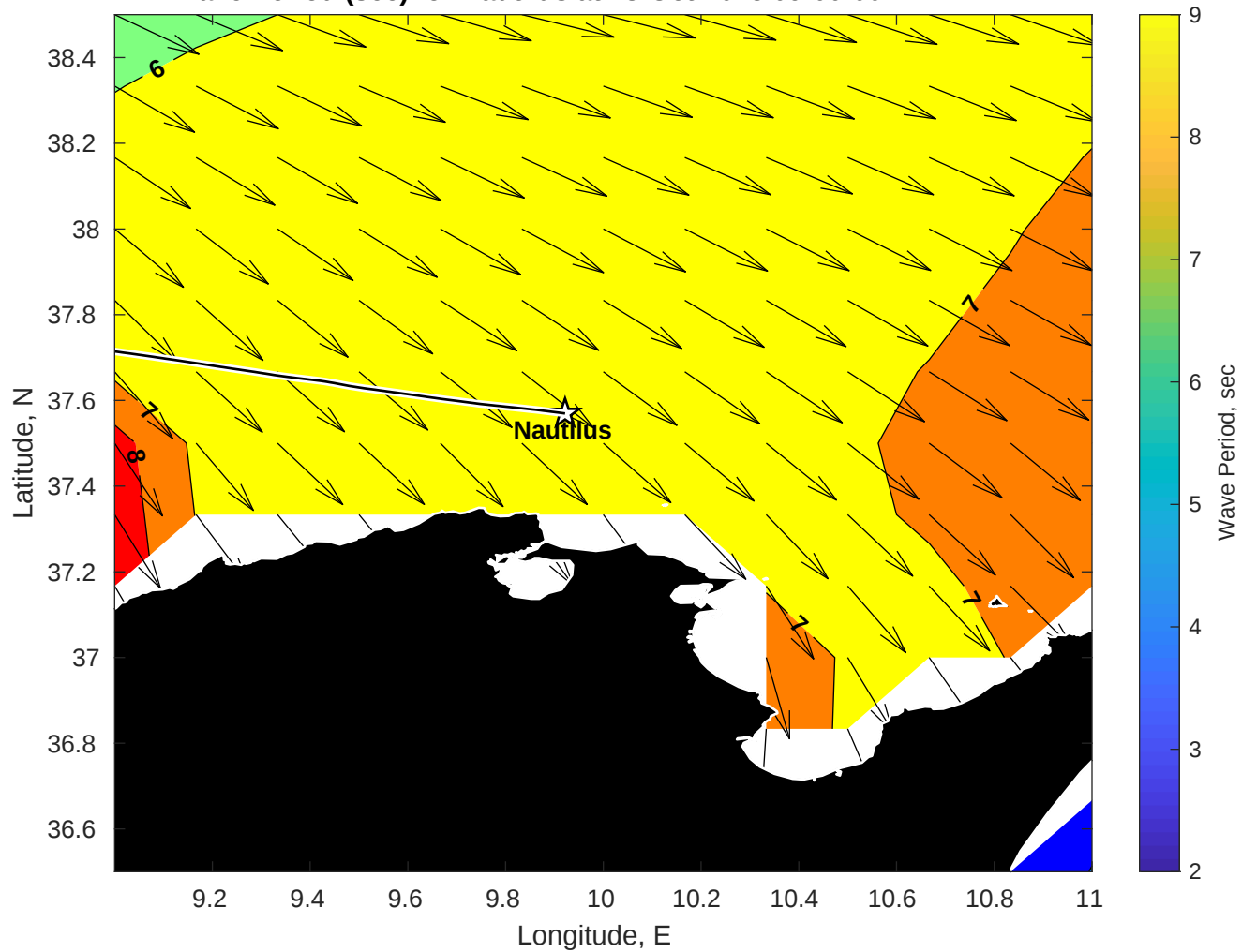
Wave Period (sec) for Nautilus at 28-Oct-2025 09:00:00
