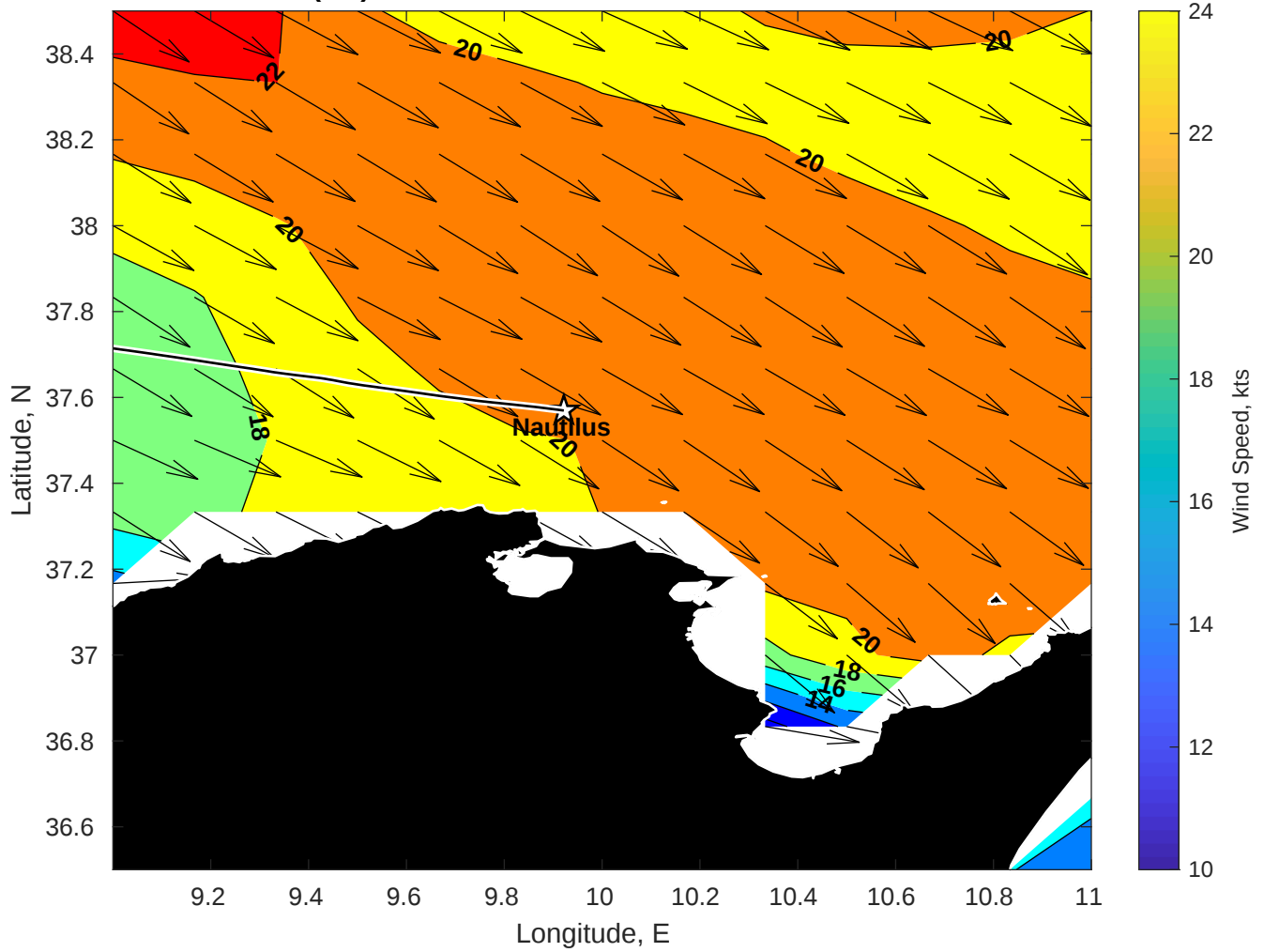
Winds (kts) for Nautilus at 28-Oct-2025 09:00:00
