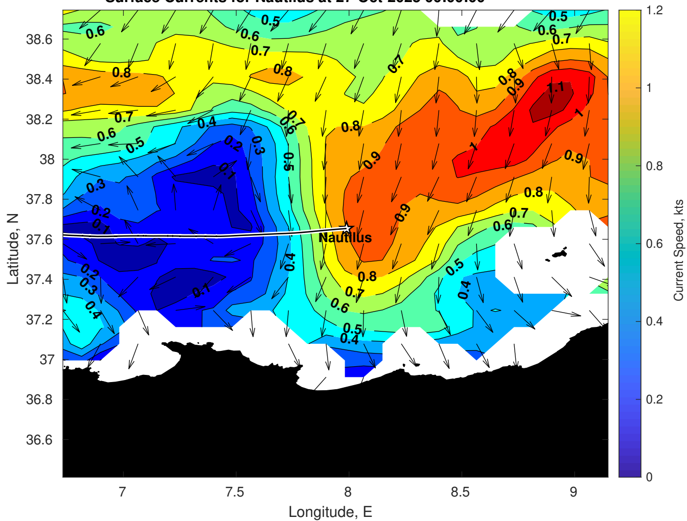
Surface Currents for Nautilus at 27-Oct-2025 00:00:00
