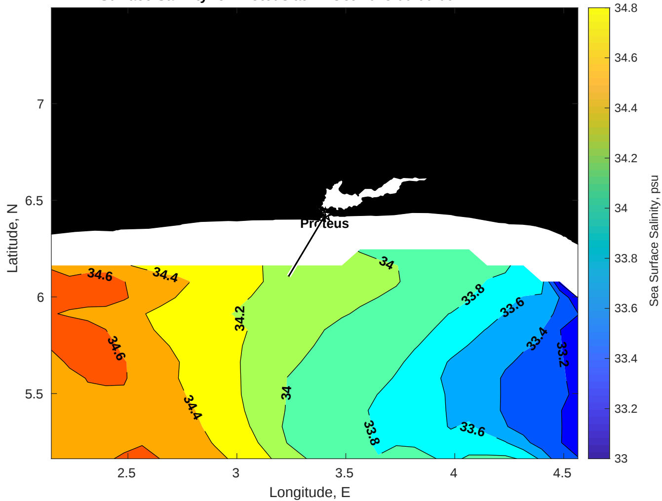
Surface Salinity for Proteus at 27-Oct-2025 00:00:00
