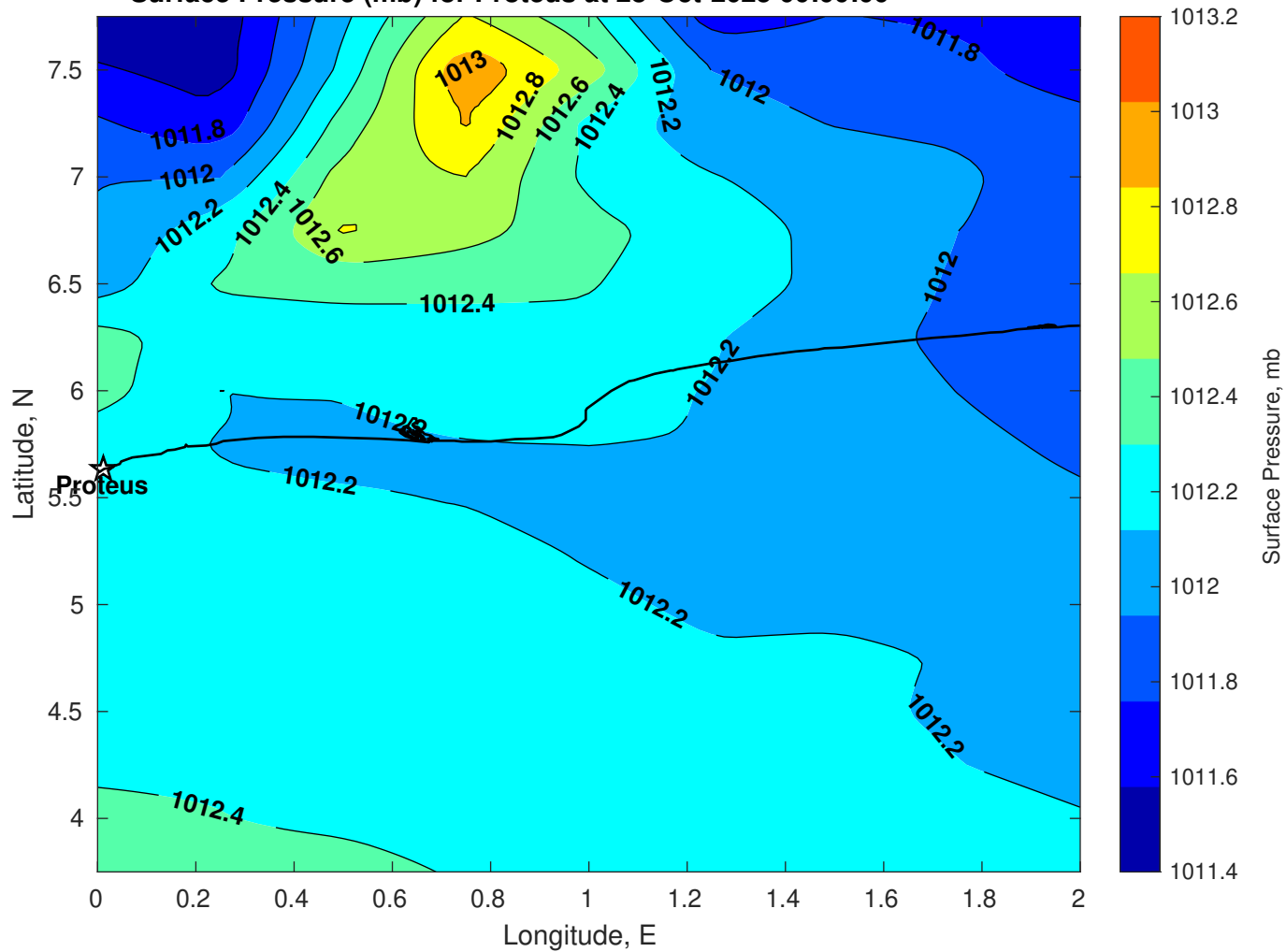
Surface Pressure (mb) for Proteus at 28-Oct-2025 00:00:00
