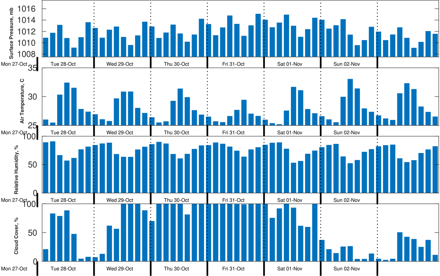
Met Forecast for Proteus from 28-Oct-2025 00:00:00 to 04-Nov-2025 00:00:00
