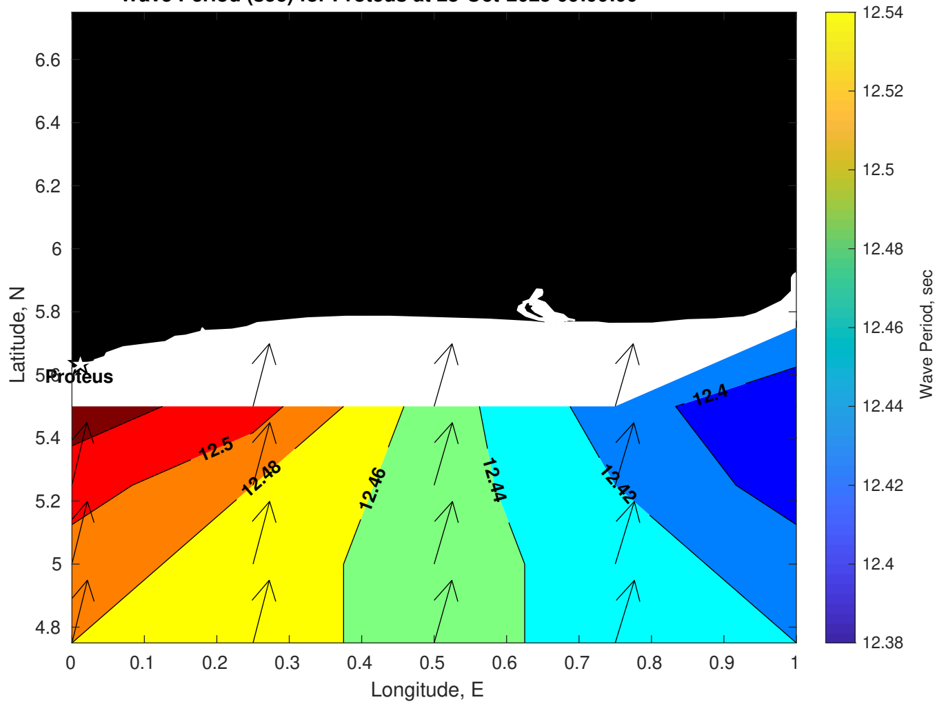
Wave Period (sec) for Proteus at 28-Oct-2025 09:00:00
