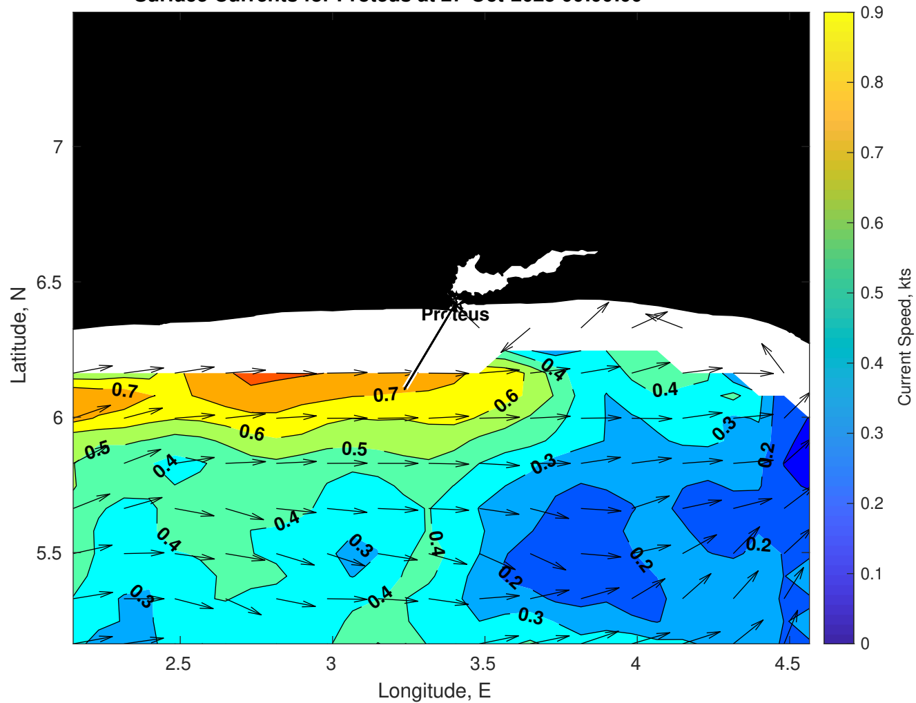
Surface Currents for Proteus at 27-Oct-2025 00:00:00
