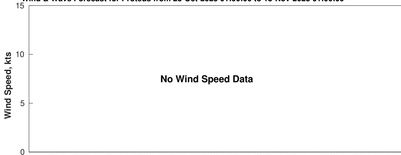
Wind & Wave Forecast for Proteus from 28-Oct-2025 01:00:00 to 13-Nov-2025 01:00:00
