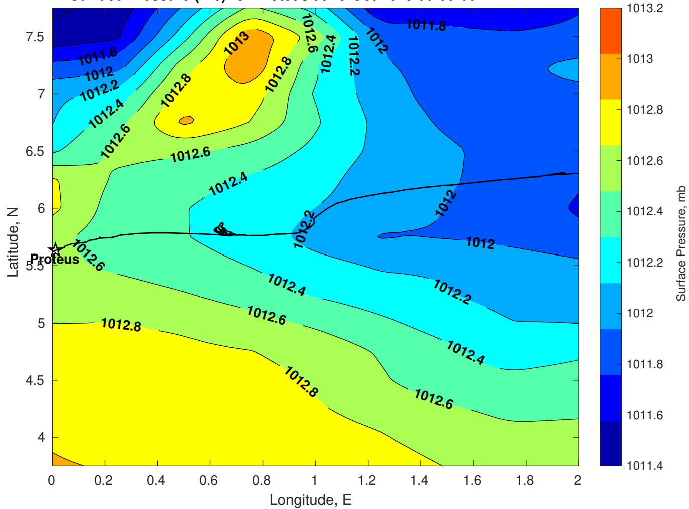
Surface Pressure (mb) for Proteus at 29-Oct-2025 00:00:00
