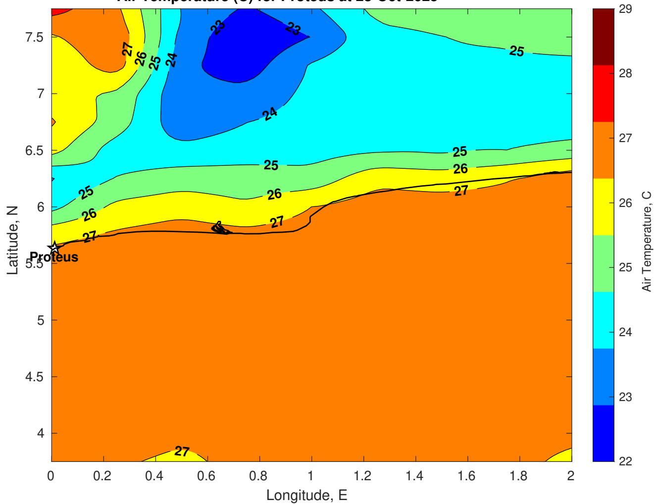
Air Temperature (C) for Proteus at 28-Oct-2025
