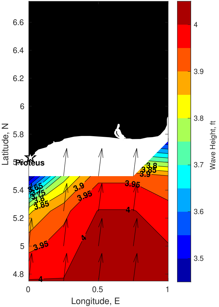
Wave Height (ft) for Proteus at 28-Oct-2025 09:00:00
