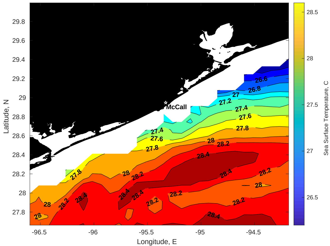
SST for Brooks McCall at 28-Oct-2025 00:00:00
