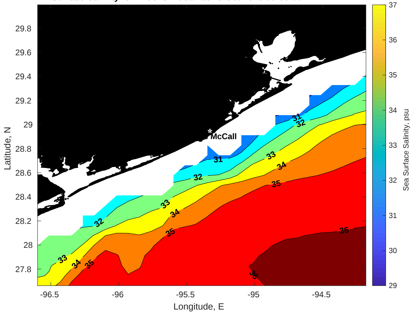
Surface Salinity for Brooks McCall at 28-Oct-2025 00:00:00
