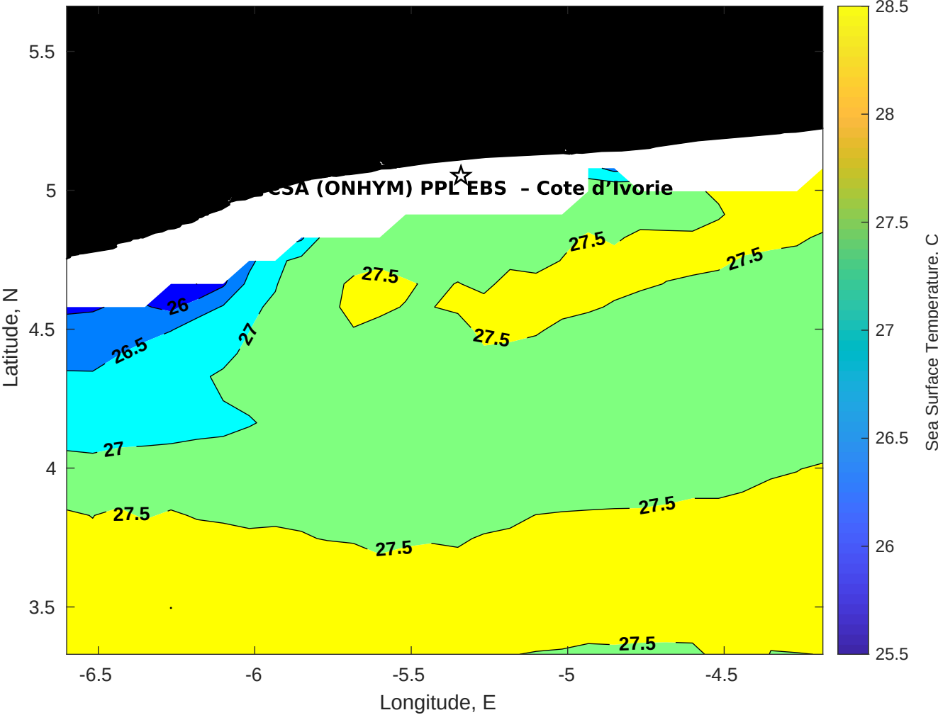
SST for CSA (ONHYM) PPL EBS - Cote d'Ivoire at 28-Oct-2025 00:00:00
