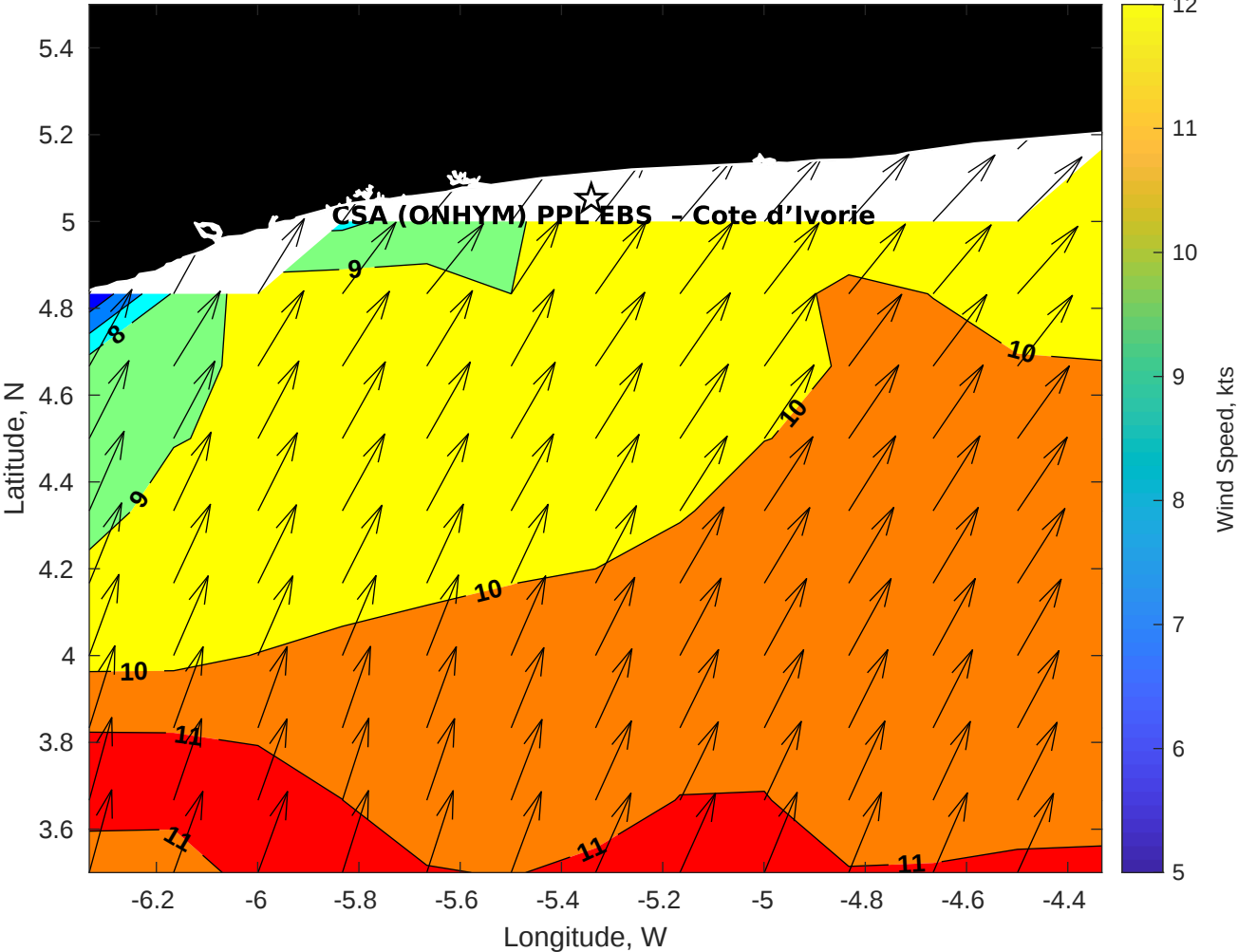
Winds (kts) for CSA (ONHYM) PPL EBS - Cote d'Ivoire at 29-Oct-2025 09:00:00
