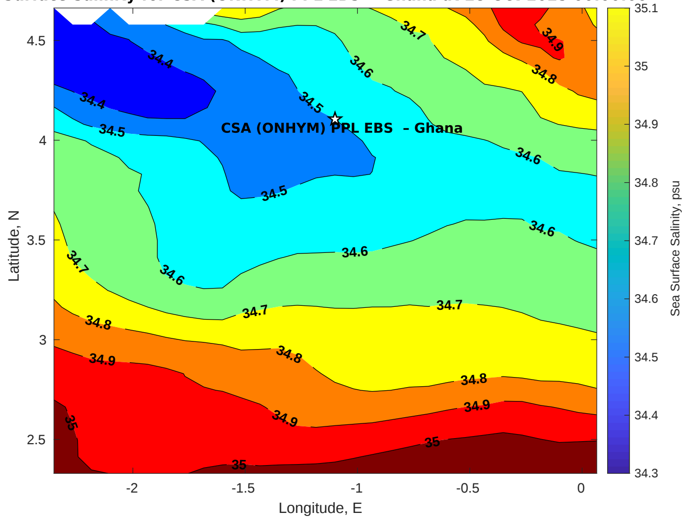
Surface Salinity for CSA (ONHYM) PPL EBS - Ghana at 28-Oct-2025 00:00:00
