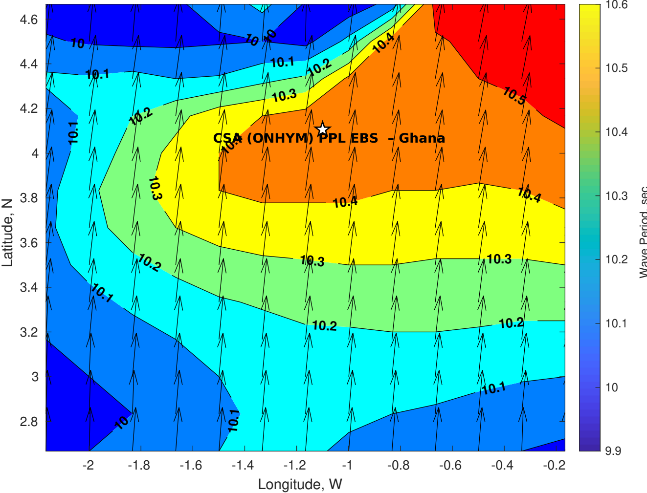
Wave Period (sec) for CSA (ONHYM) PPL EBS - Ghana at 29-Oct-2025 09:00:00
