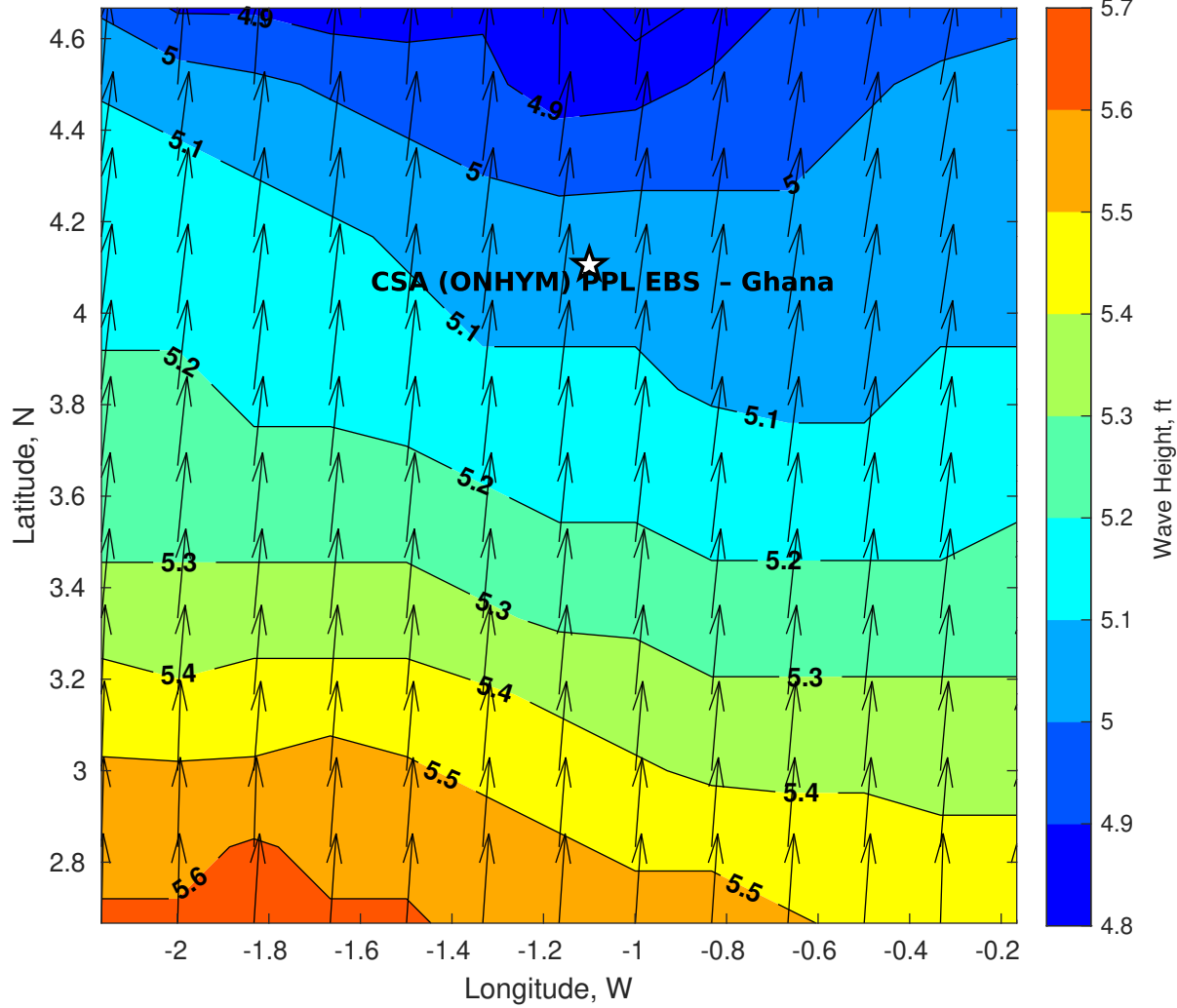
Wave Height (ft) for CSA (ONHYM) PPL EBS - Ghana at 29-Oct-2025 09:00:00
