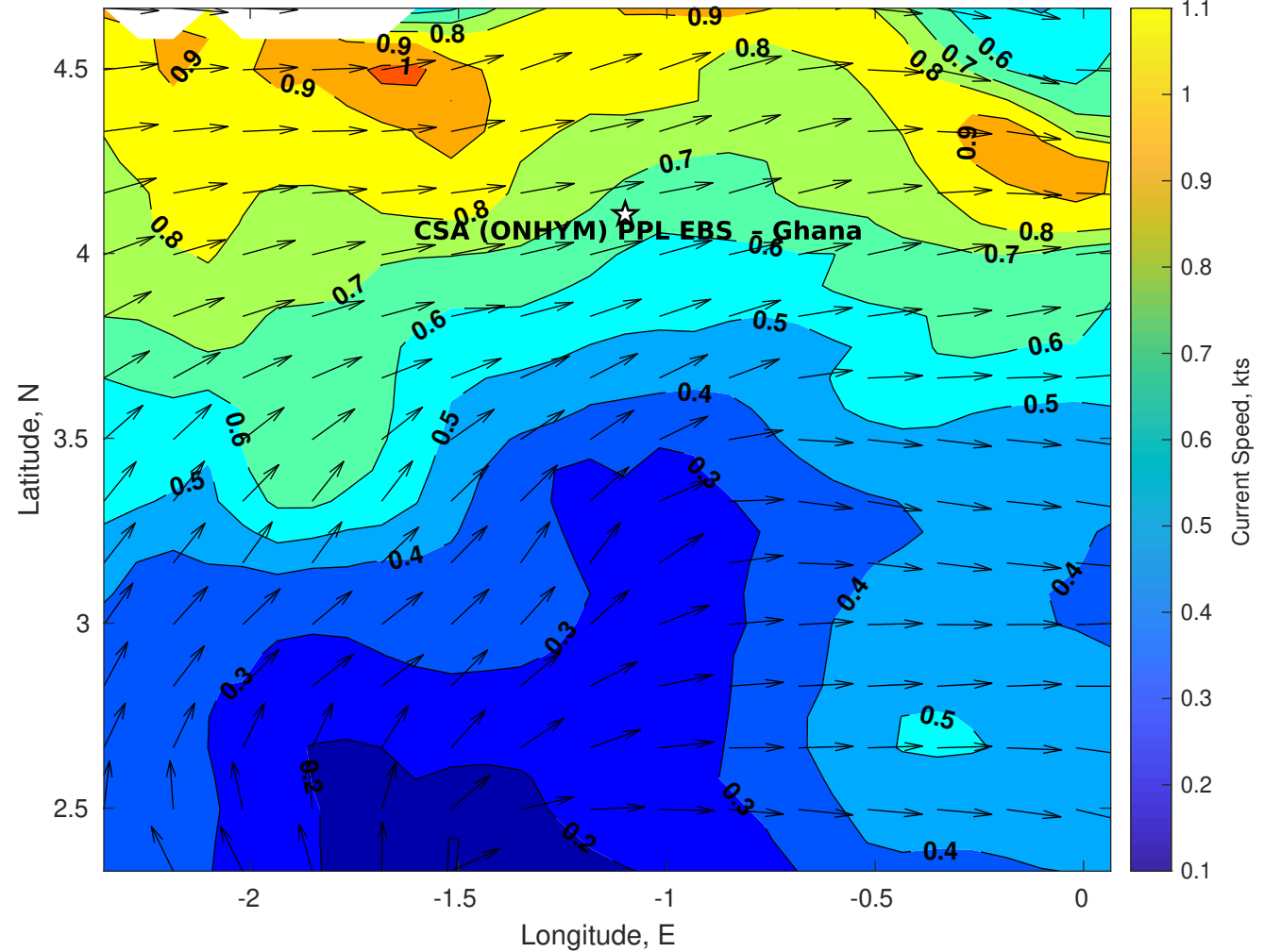
Surface Currents for CSA (ONHYM) PPL EBS - Ghana at 28-Oct-2025 00:00:00
