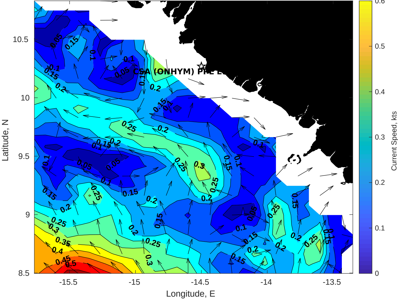
Surface Currents for CSA (ONHYM) PPL EBS - Guinea at 28-Oct-2025 00:00:00
