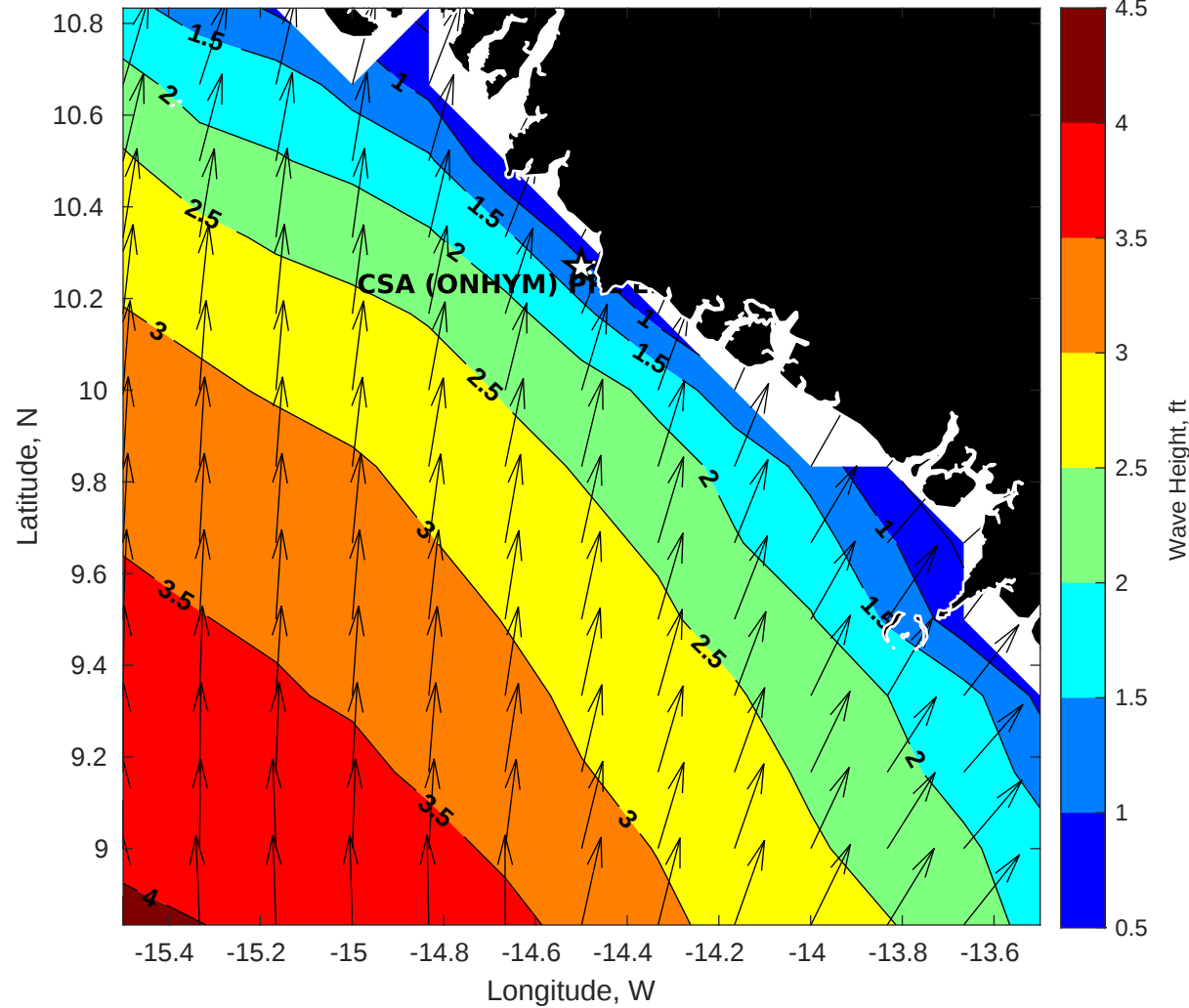
Wave Height (ft) for CSA (ONHYM) PPL EBS - Guinea at 29-Oct-2025 09:00:00
