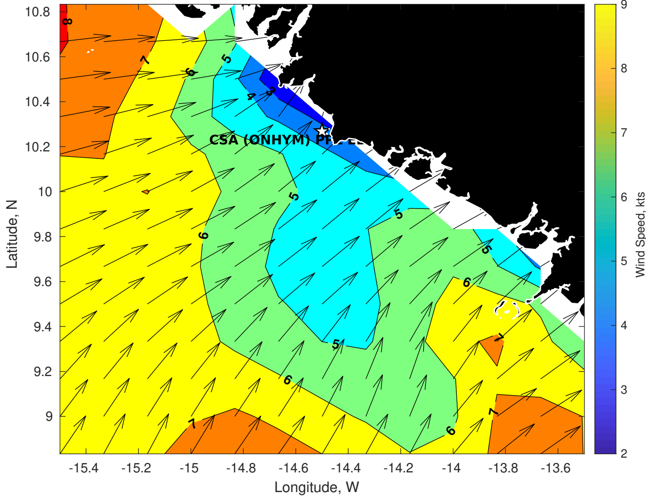
Winds (kts) for CSA (ONHYM) PPL EBS - Guinea at 29-Oct-2025 09:00:00
