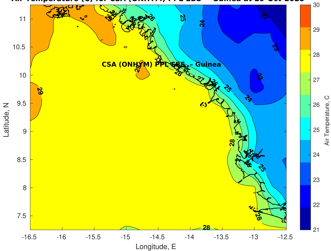
Air Temperature (C) for CSA (ONHYM) PPL EBS - Guinea at 29-Oct-2025
