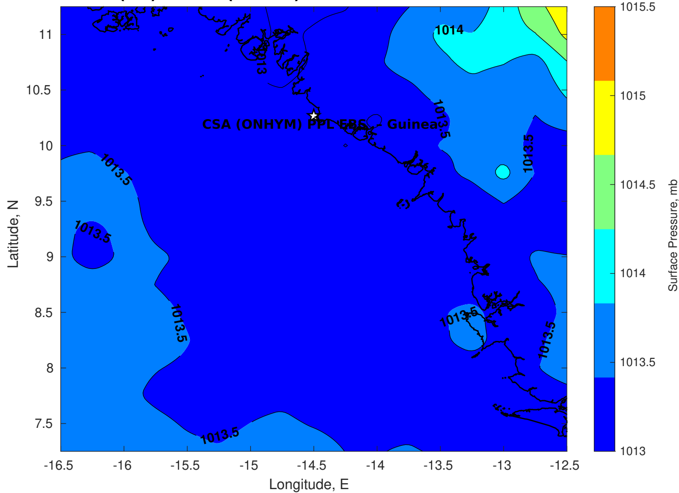
Surface Pressure (mb) for CSA (ONHYM) PPL EBS - Guinea at 29-Oct-2025 00:00:00
