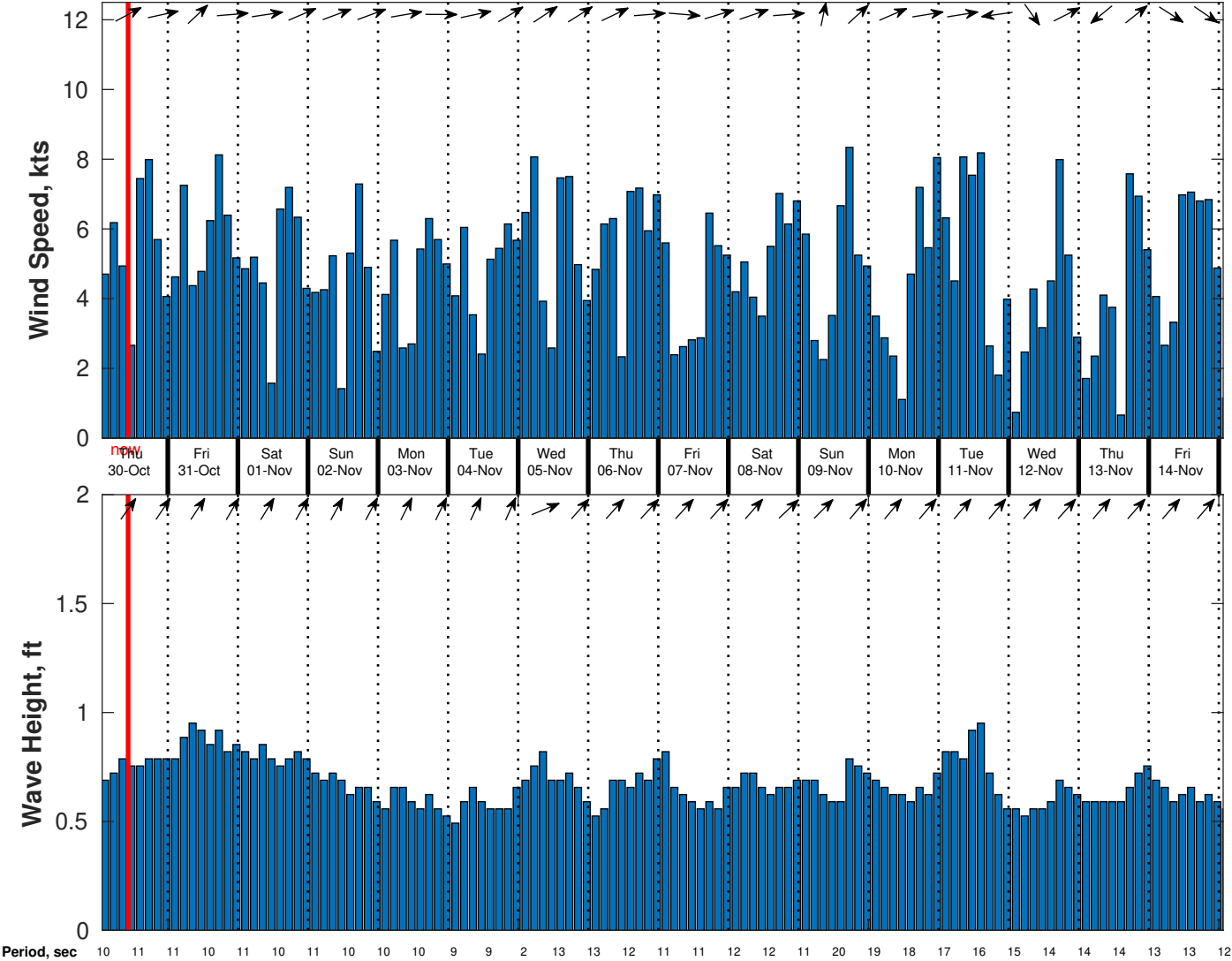
Wind & Wave Forecast for CSA (ONHYM) PPL EBS - Guinea from 29-Oct-2025 01:00:00 to 14-Nov-2025 01:00:00
