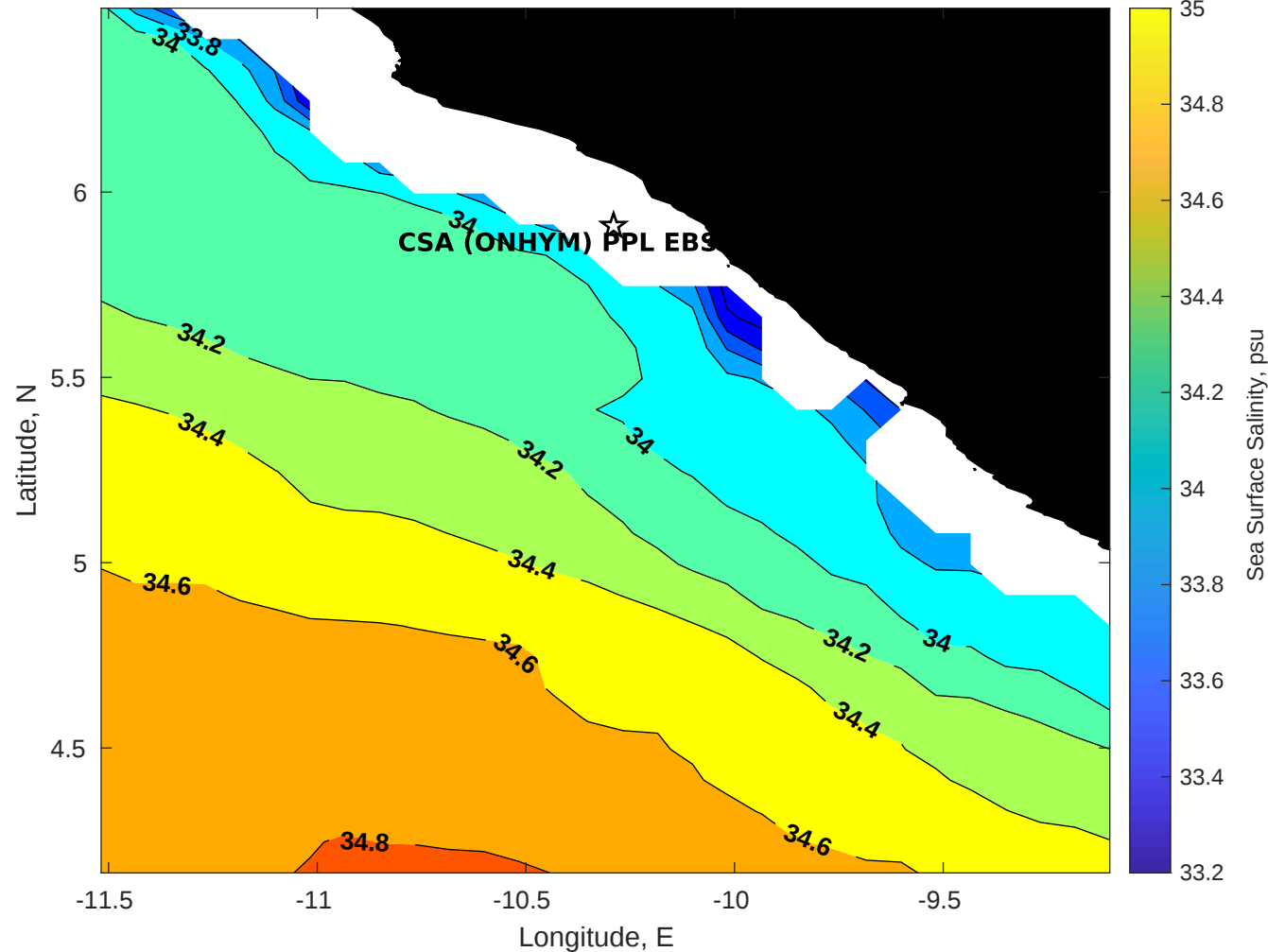
Surface Salinity for CSA (ONHYM) PPL EBS - Liberia at 28-Oct-2025 00:00:00
