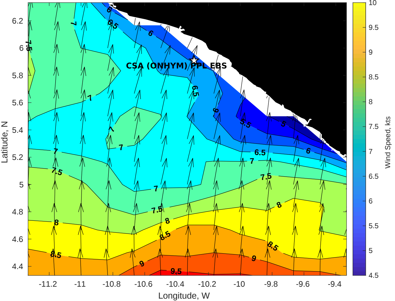
Winds (kts) for CSA (ONHYM) PPL EBS - Liberia at 29-Oct-2025 09:00:00
