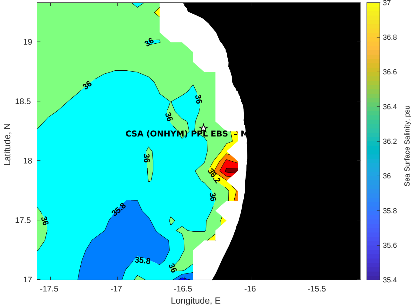
Surface Salinity for CSA (ONHYM) PPL EBS - Mauritania at 28-Oct-2025 00:00:00
