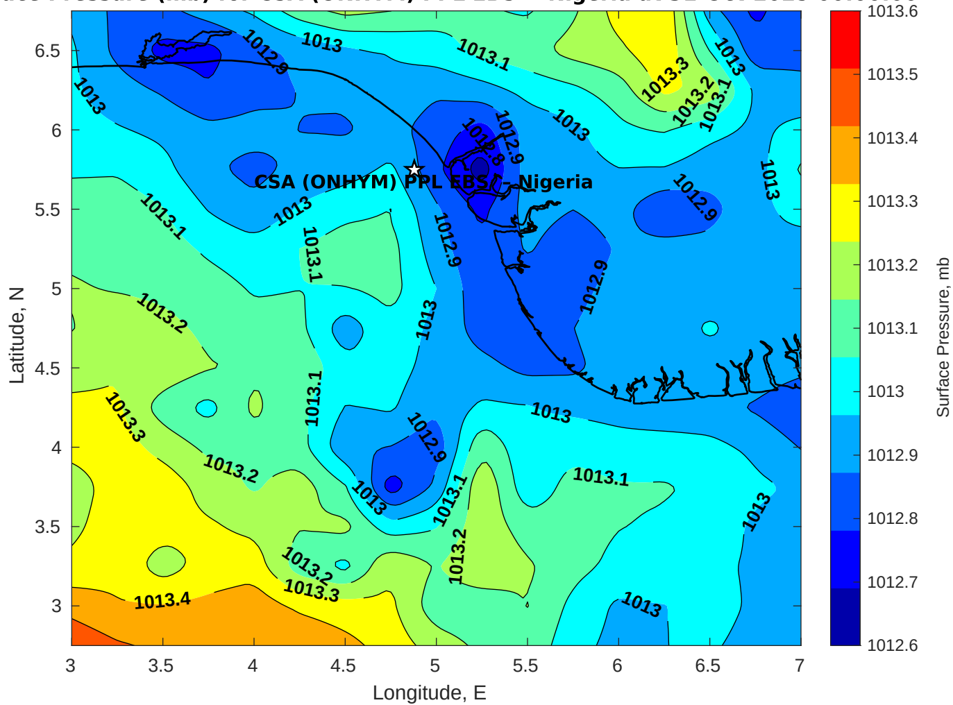
Surface Pressure (mb) for CSA (ONHYM) PPL EBS - Nigeria at 31-Oct-2025 00:00:00
