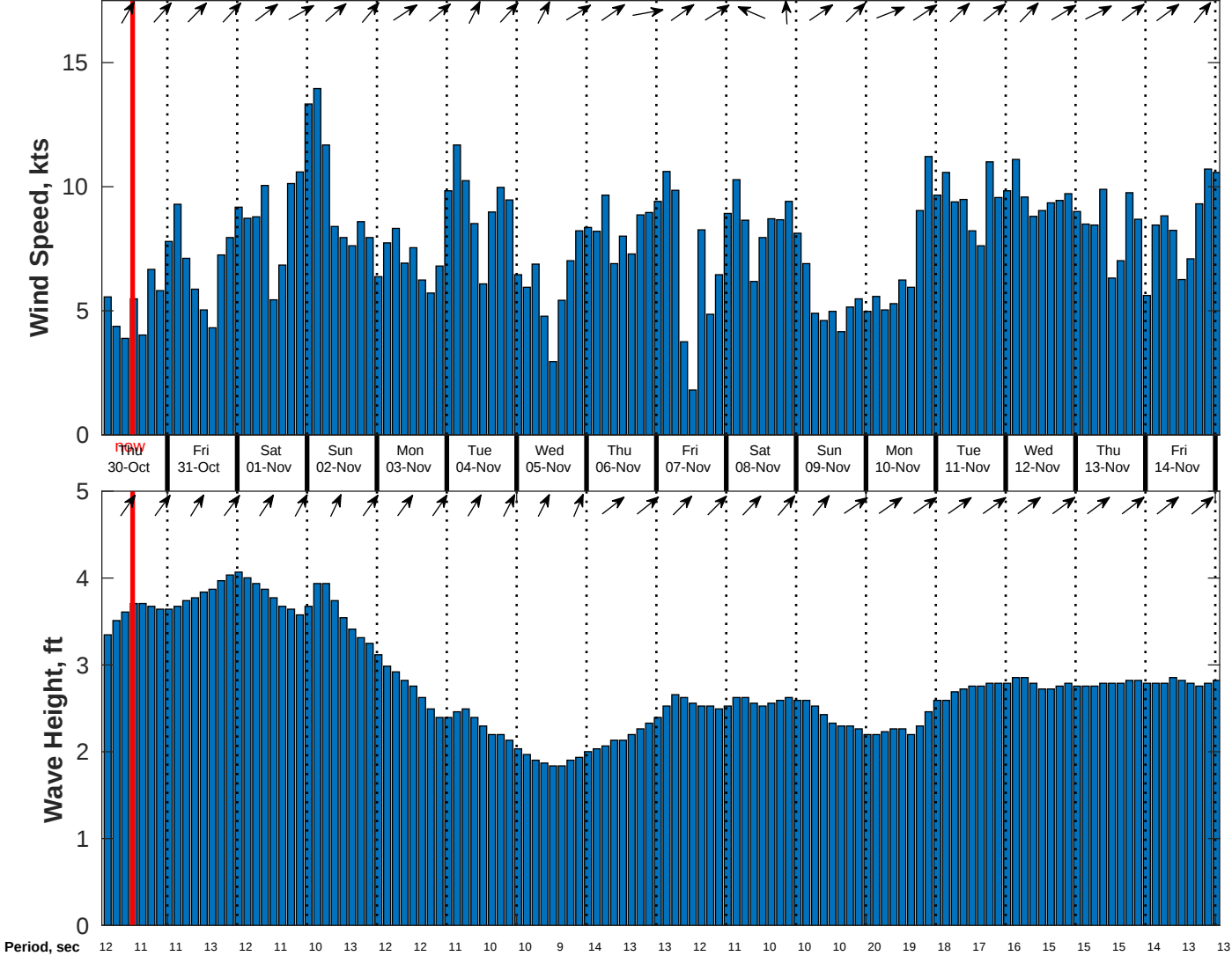
Wind & Wave Forecast for CSA (ONHYM) PPL EBS - Nigeria from 29-Oct-2025 02:00:00 to 14-Nov-2025 02:00:00
