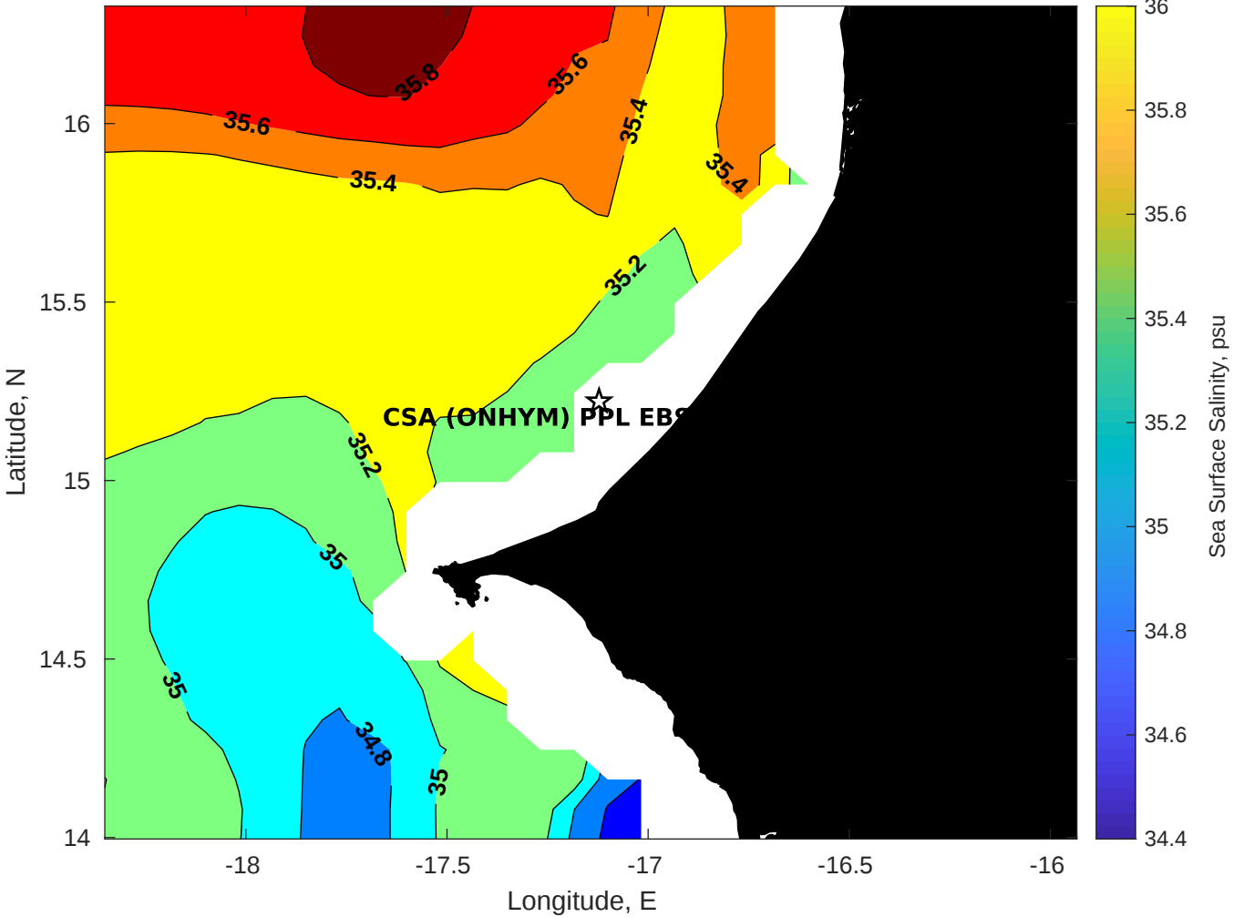
Surface Salinity for CSA (ONHYM) PPL EBS - Senegal at 28-Oct-2025 00:00:00
