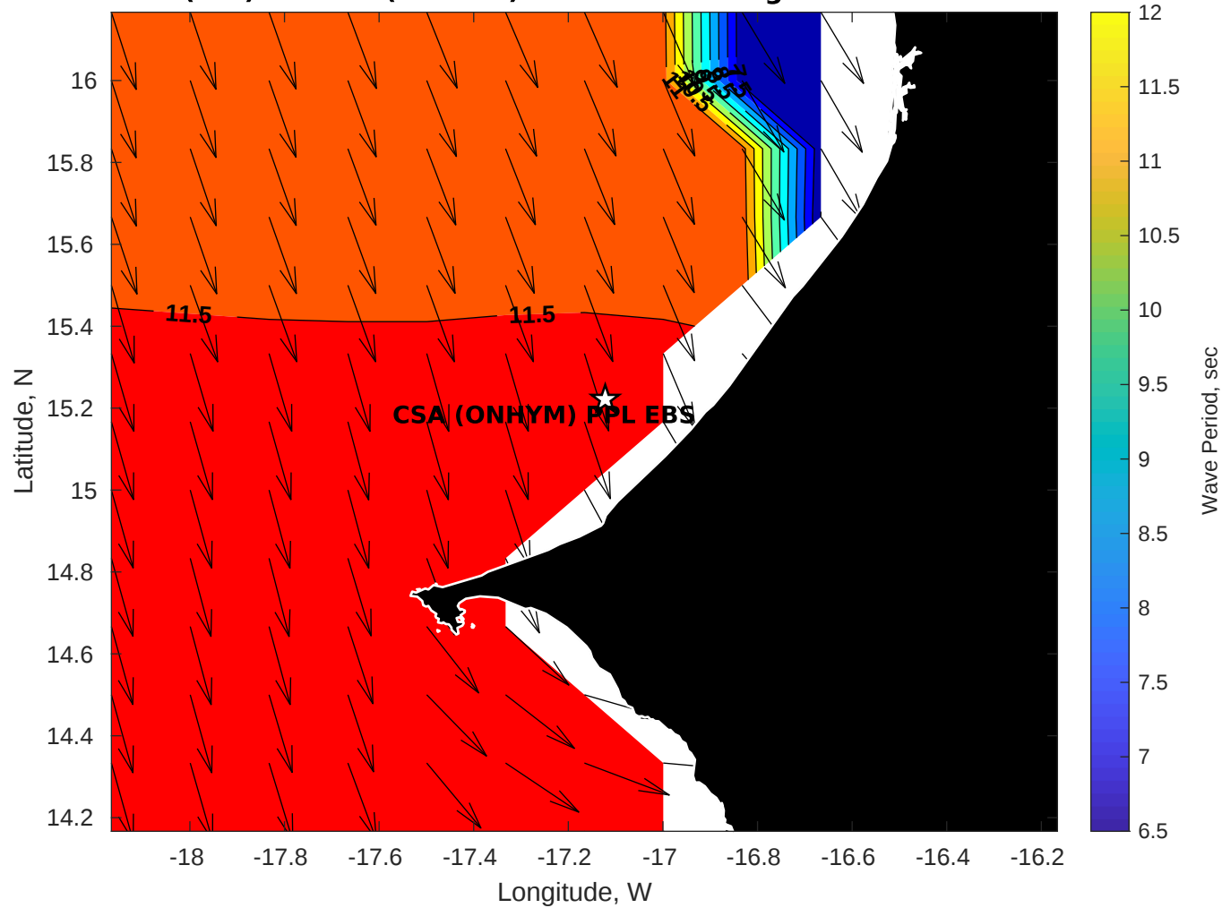
Wave Period (sec) for CSA (ONHYM) PPL EBS - Senegal at 29-Oct-2025 09:00:00
