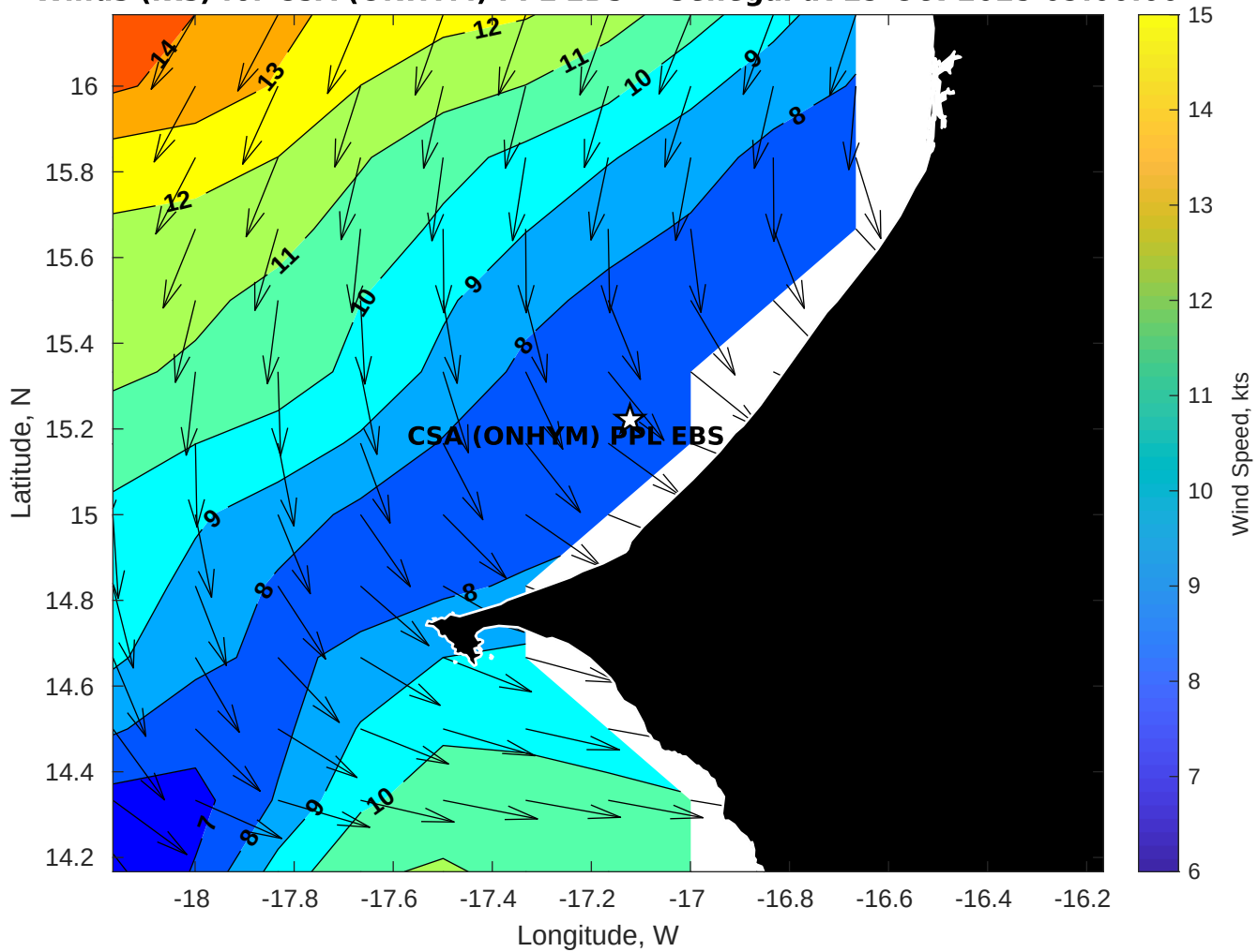
Winds (kts) for CSA (ONHYM) PPL EBS - Senegal at 29-Oct-2025 09:00:00
