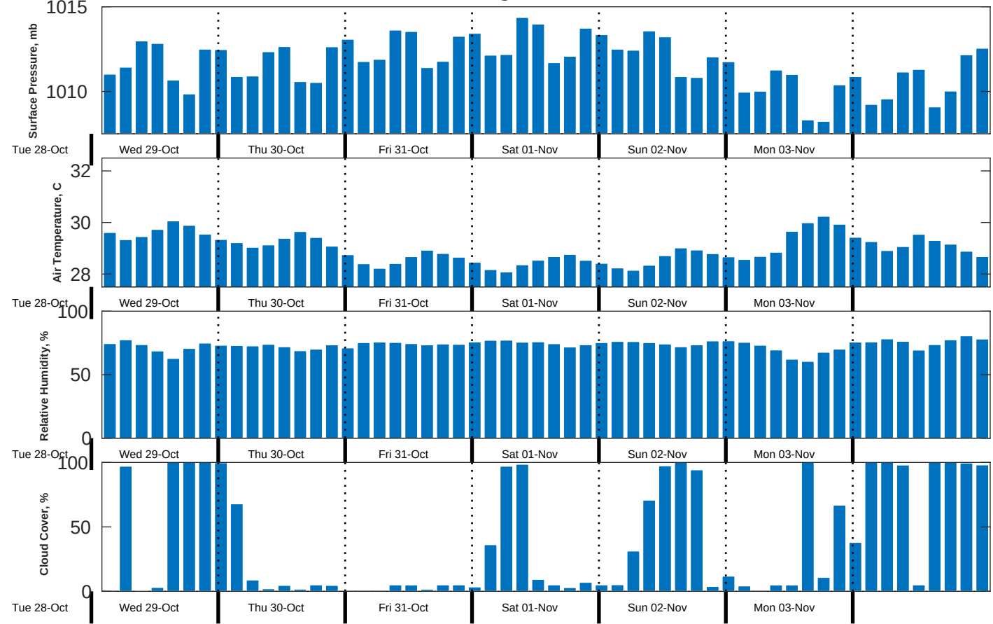
Met Forecast for CSA (ONHYM) PPL EBS - Senegal from 29-Oct-2025 00:00:00 to 05-Nov-2025 00:00:00
