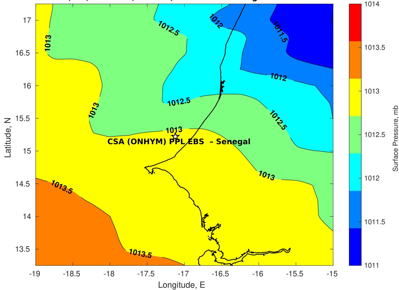
Surface Pressure (mb) for CSA (ONHYM) PPL EBS - Senegal at 31-Oct-2025 00:00:00
