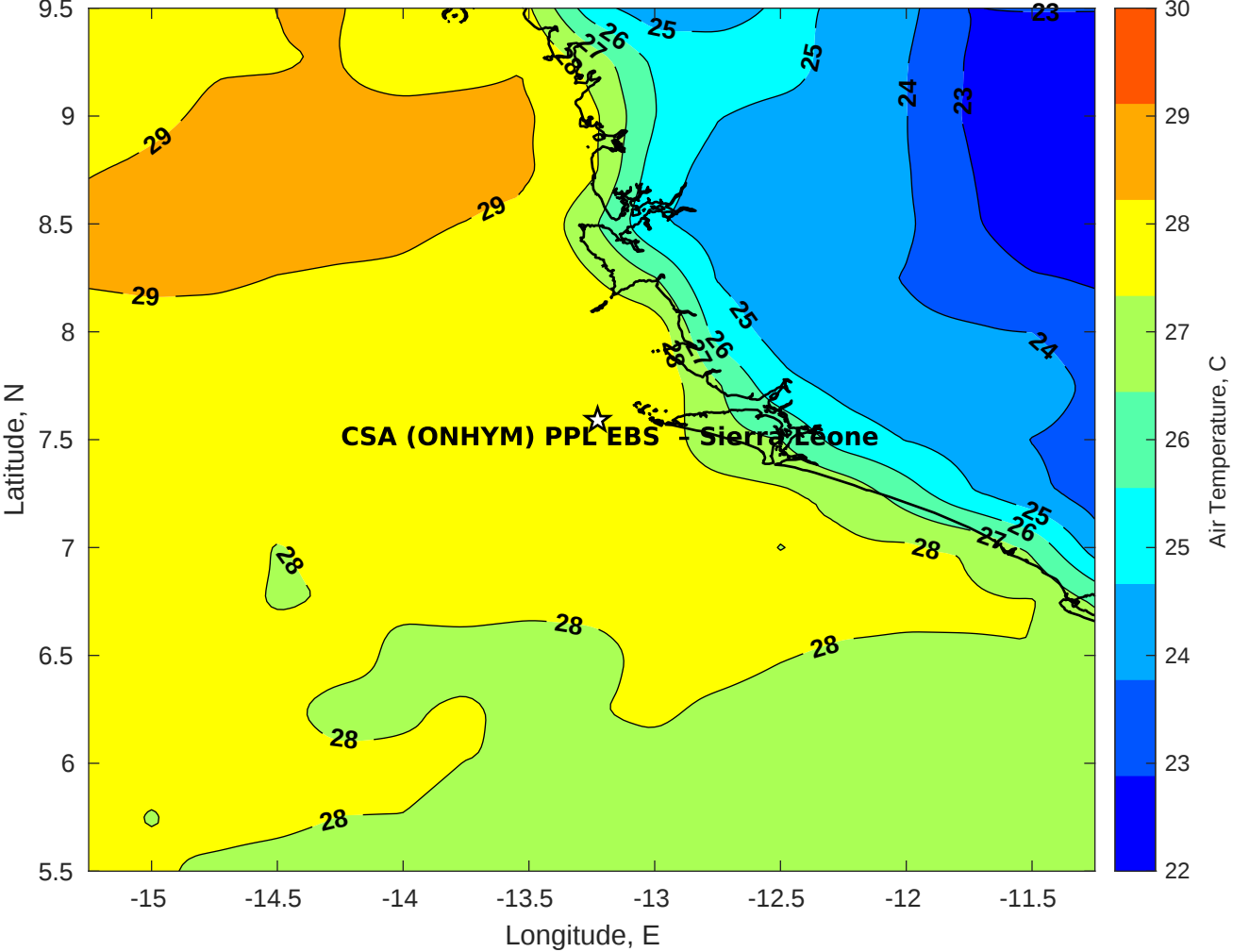
Air Temperature (C) for CSA (ONHYM) PPL EBS - Sierra Leone at 29-Oct-2025
