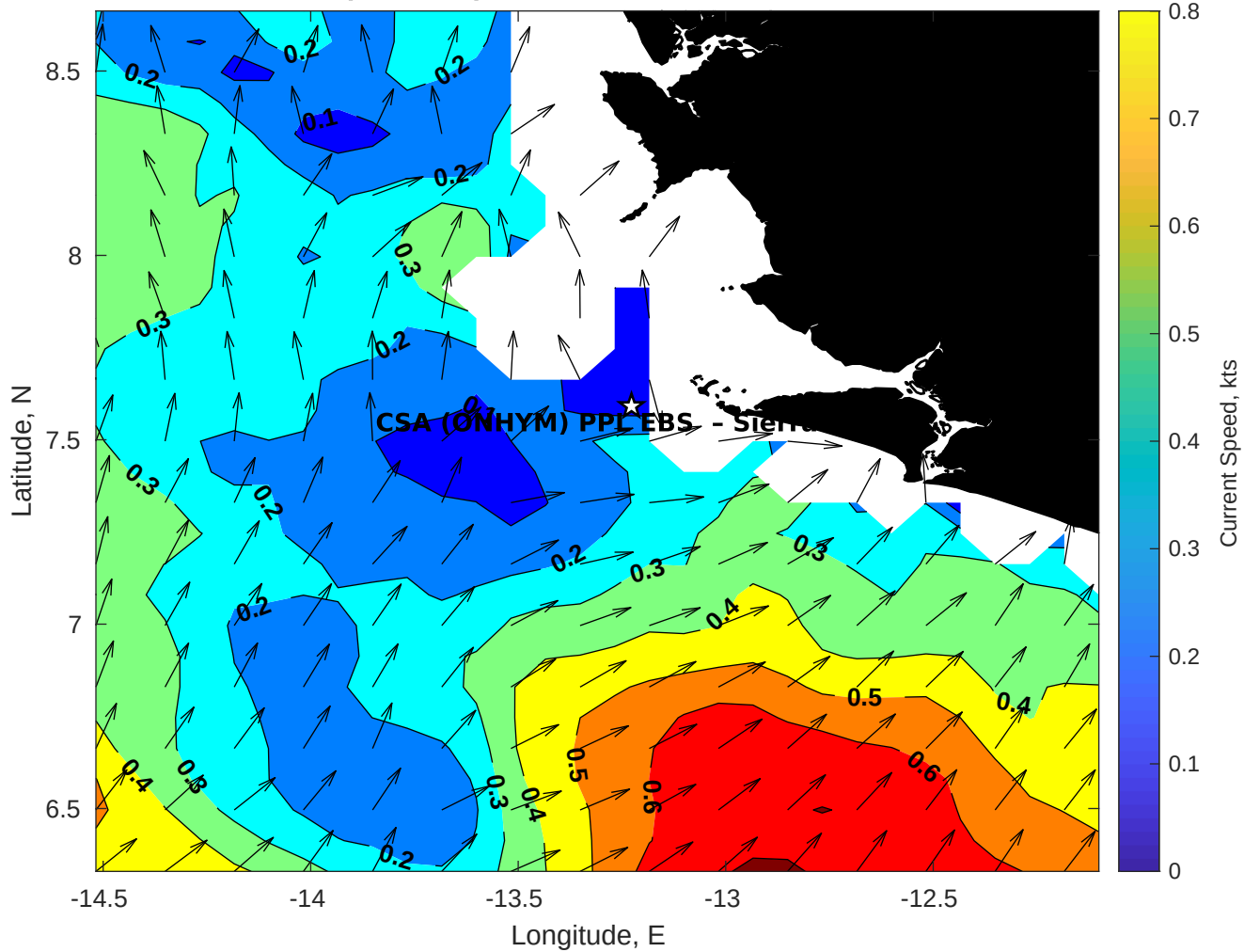
Surface Currents for CSA (ONHYM) PPL EBS - Sierra Leone at 28-Oct-2025 00:00:00
