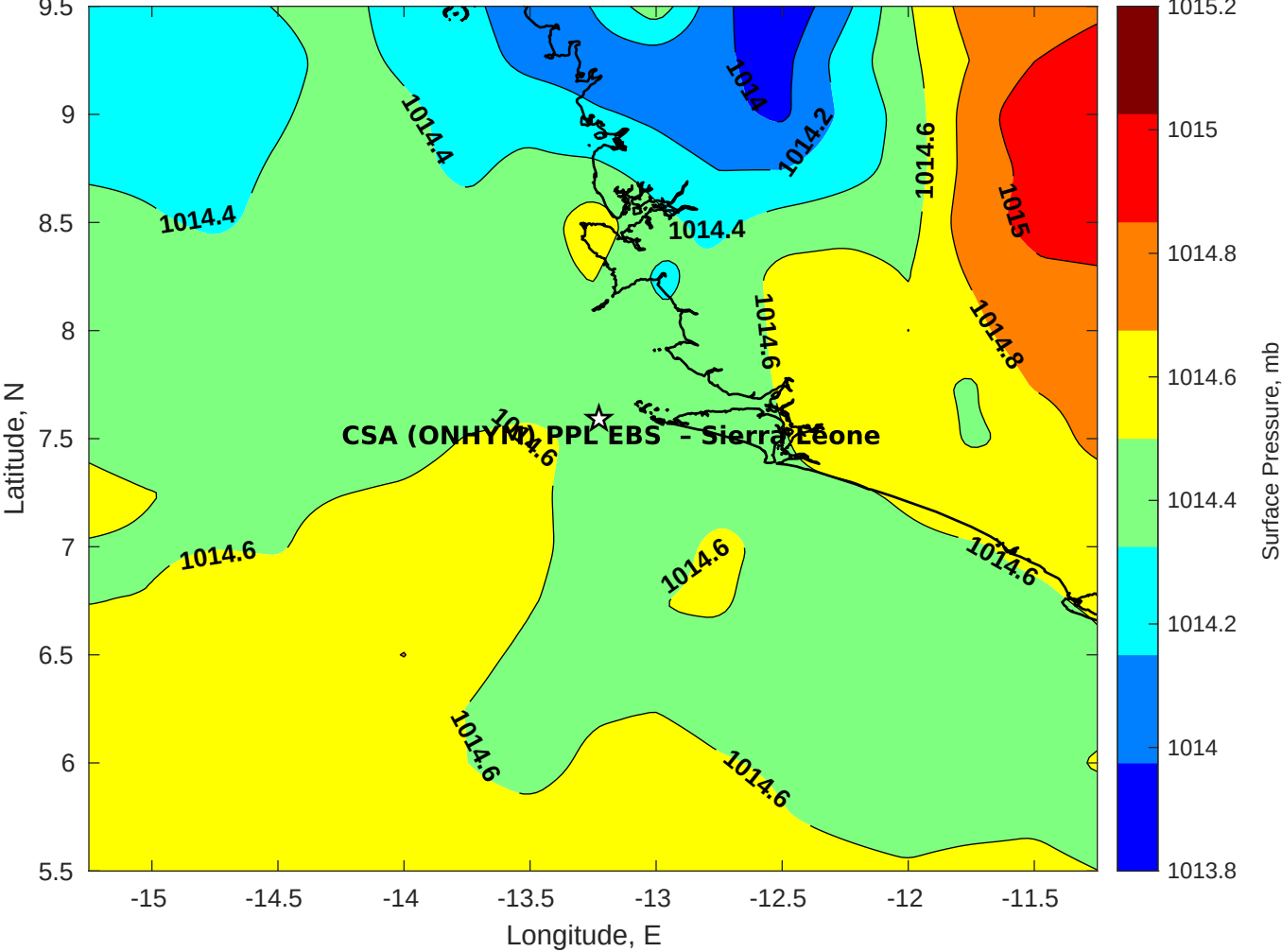
Surface Pressure (mb) for CSA (ONHYM) PPL EBS - Sierra Leone at 31-Oct-2025 00:00:00
