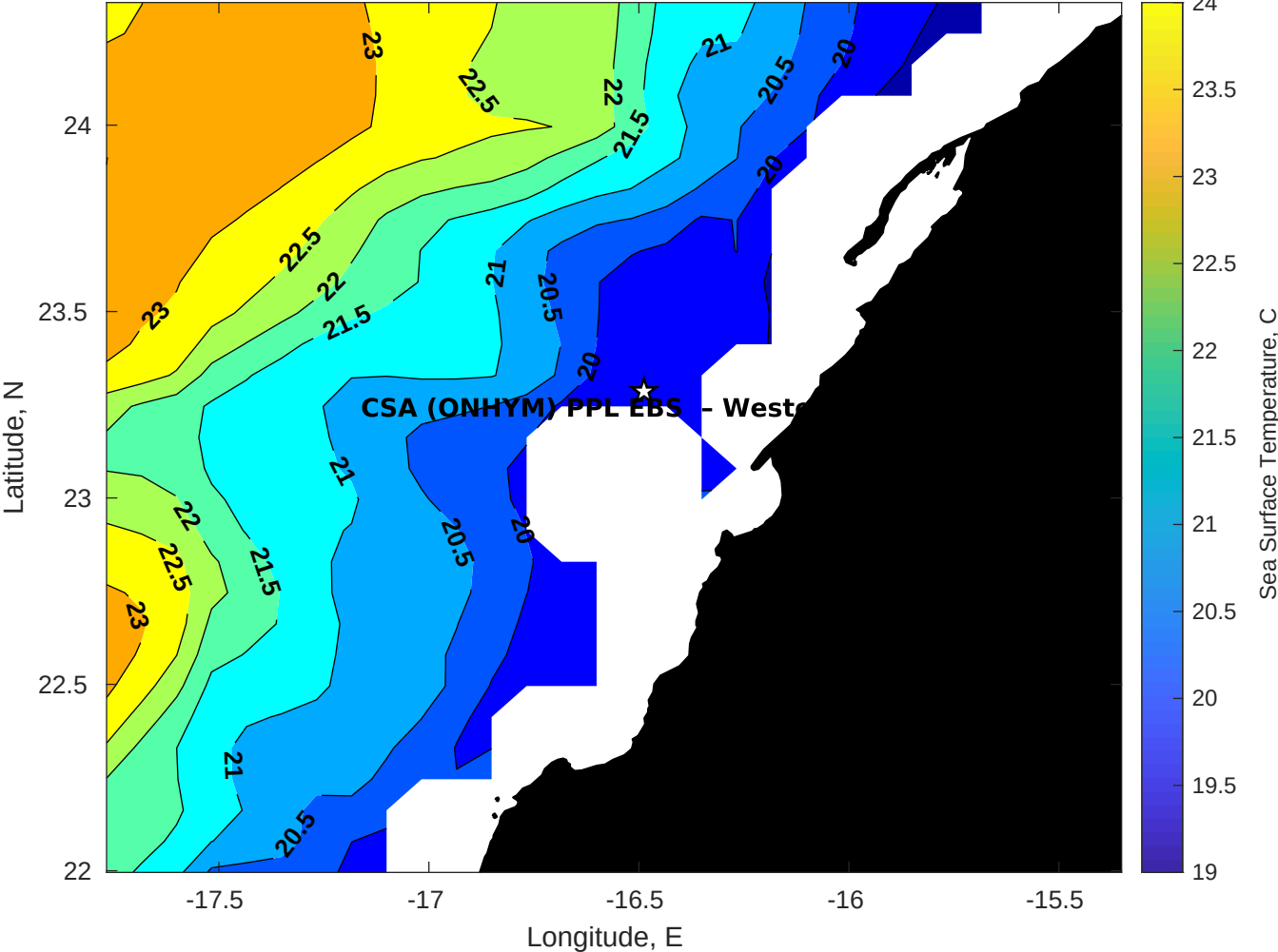
SST for CSA (ONHYM) PPL EBS - Western Sahara at 28-Oct-2025 00:00:00
