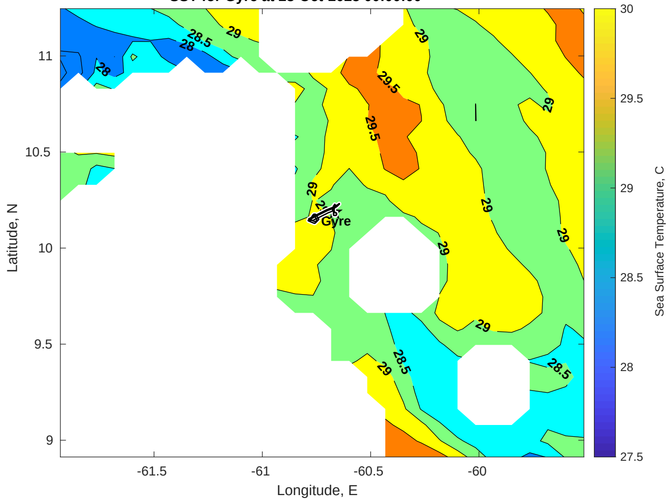
SST for Gyre at 28-Oct-2025 00:00:00
