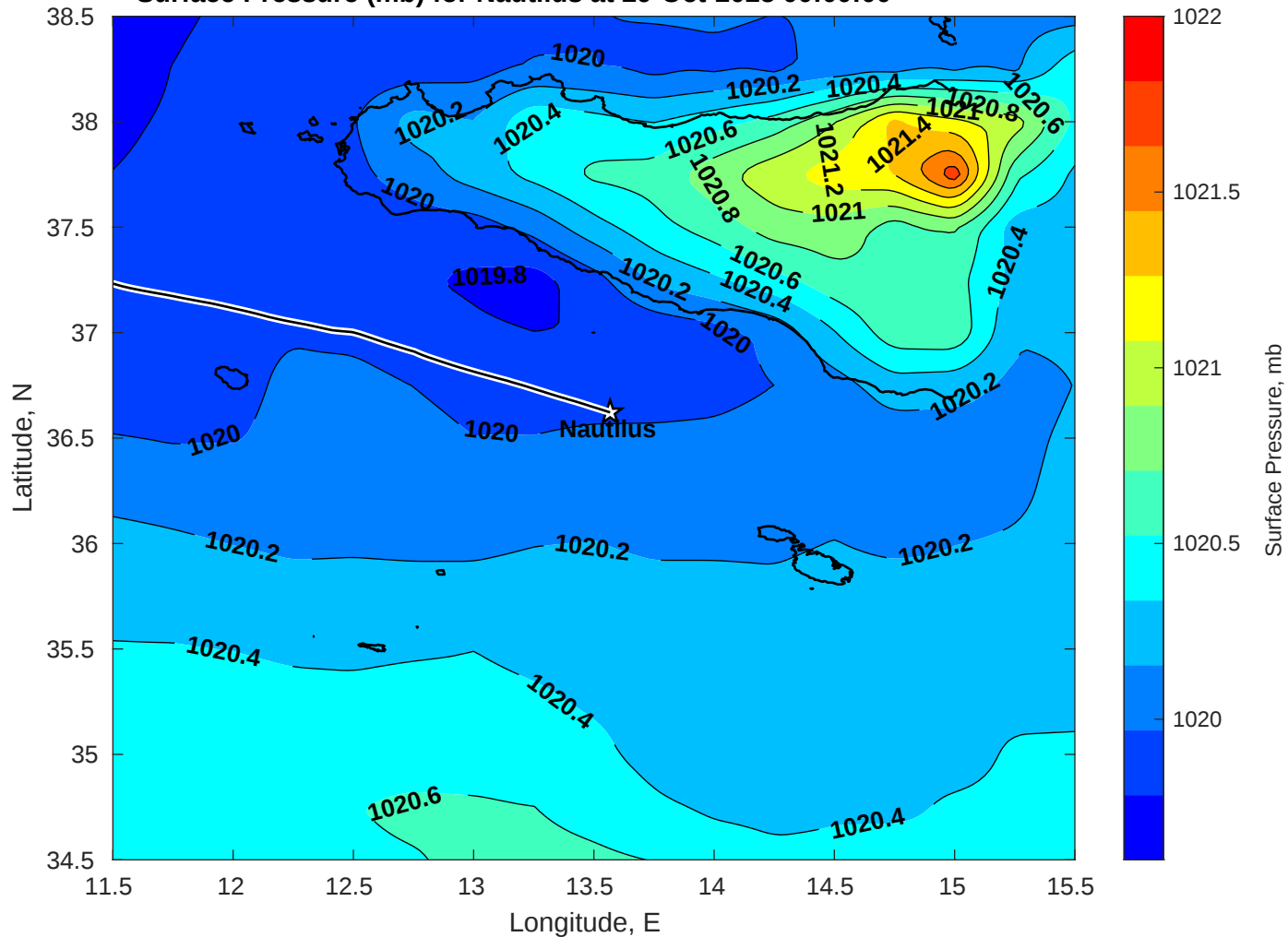
Surface Pressure (mb) for Nautilus at 29-Oct-2025 00:00:00
