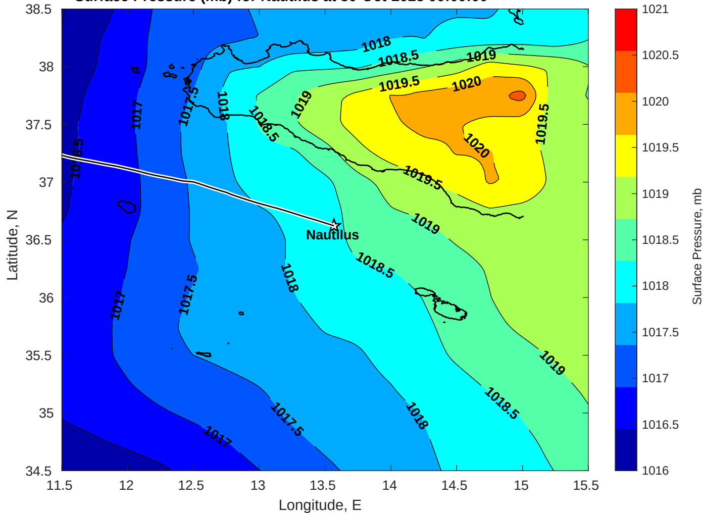
Surface Pressure (mb) for Nautilus at 30-Oct-2025 00:00:00
