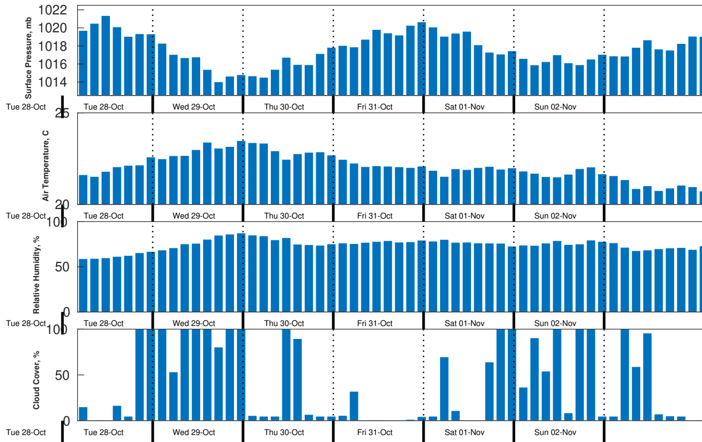
Met Forecast for Nautilus from 29-Oct-2025 00:00:00 to 05-Nov-2025 00:00:00
