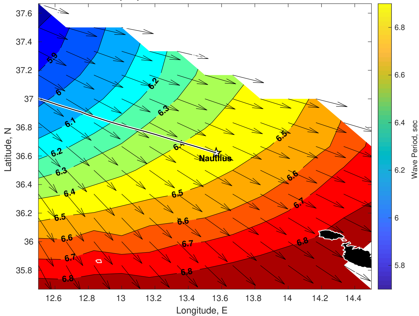
Wave Period (sec) for Nautilus at 29-Oct-2025 09:00:00
