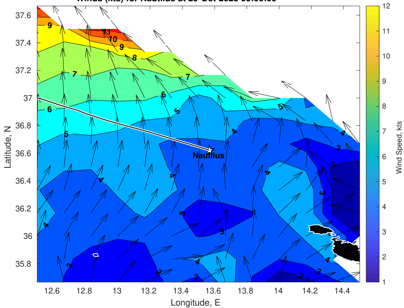
Winds (kts) for Nautilus at 29-Oct-2025 09:00:00
