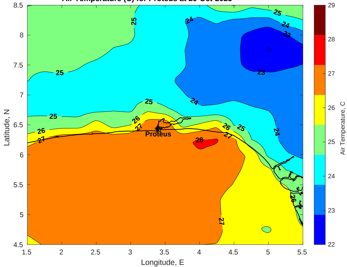
Air Temperature (C) for Proteus at 29-Oct-2025
