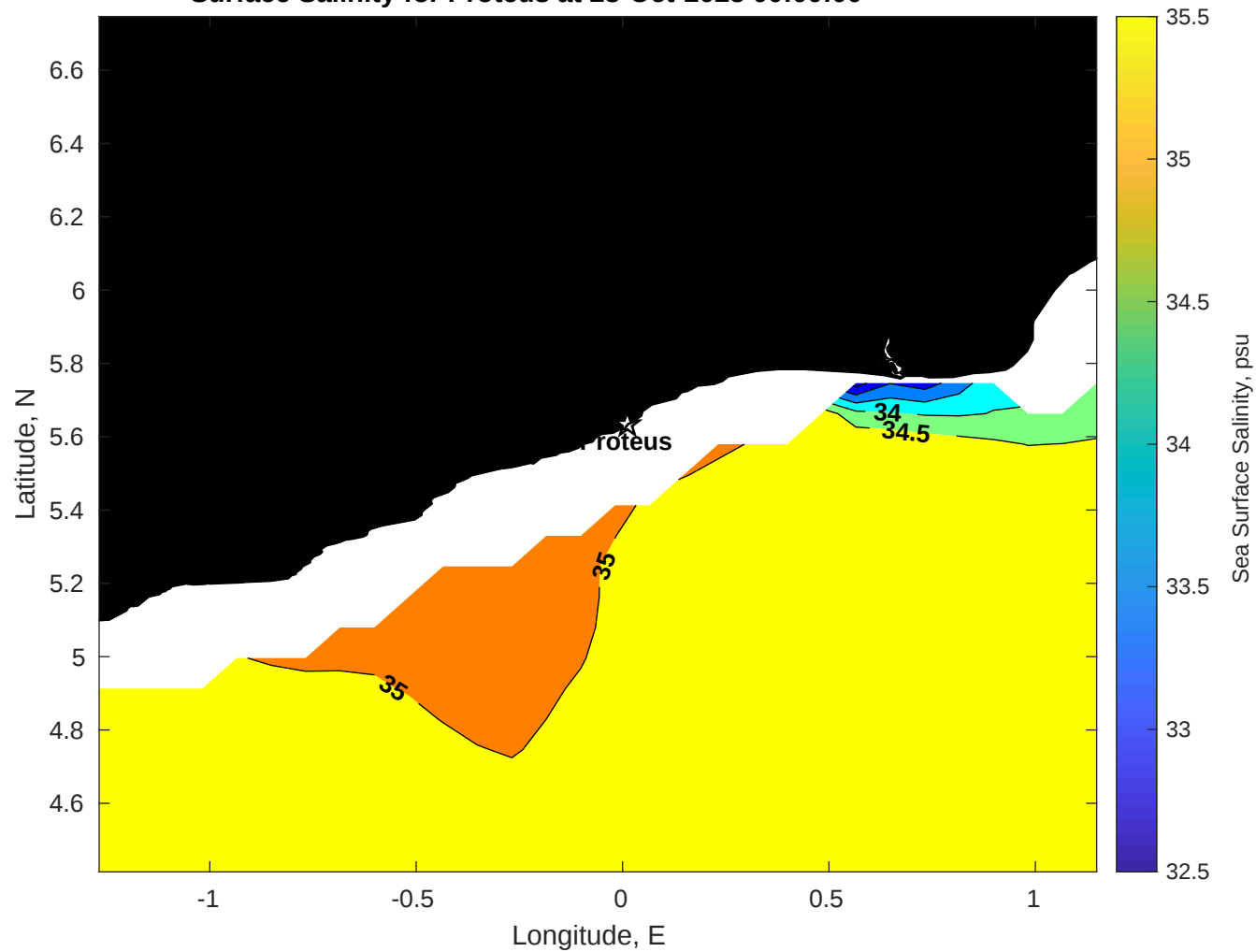
Surface Salinity for Proteus at 28-Oct-2025 00:00:00
