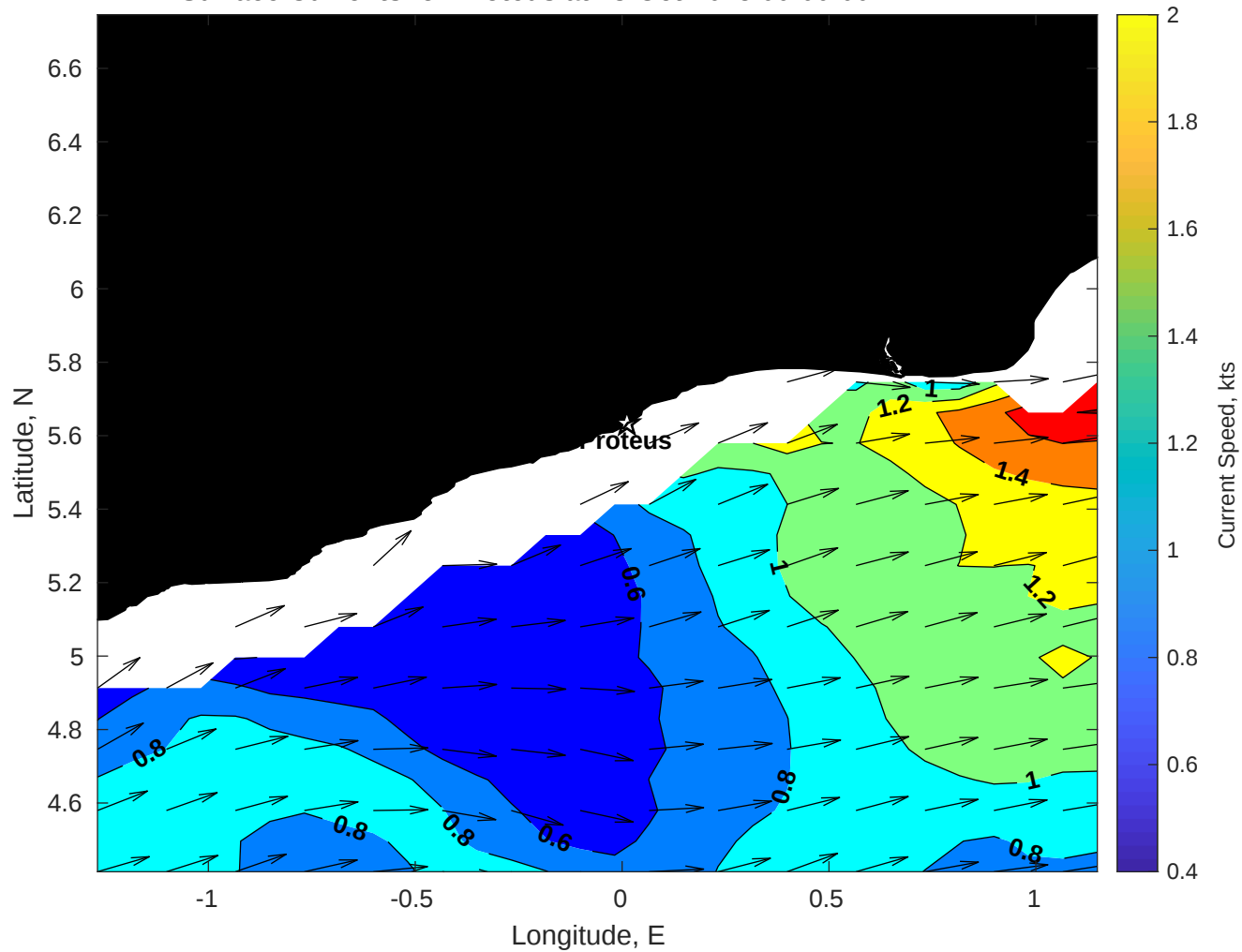
Surface Currents for Proteus at 28-Oct-2025 00:00:00
