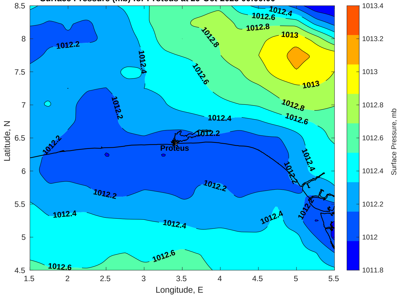
Surface Pressure (mb) for Proteus at 29-Oct-2025 00:00:00
