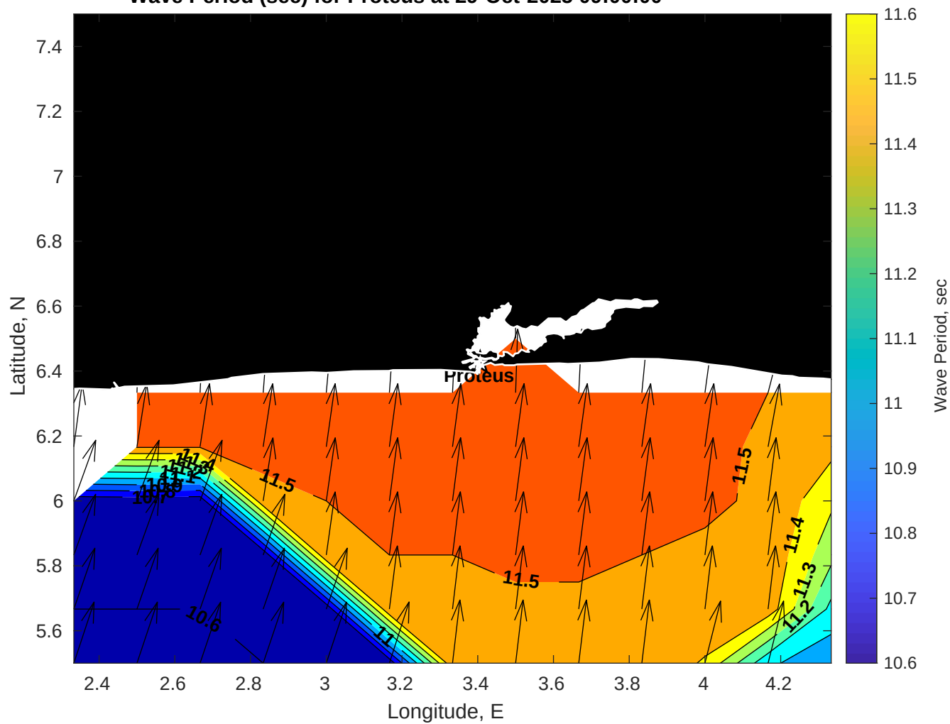
Wave Period (sec) for Proteus at 29-Oct-2025 09:00:00
