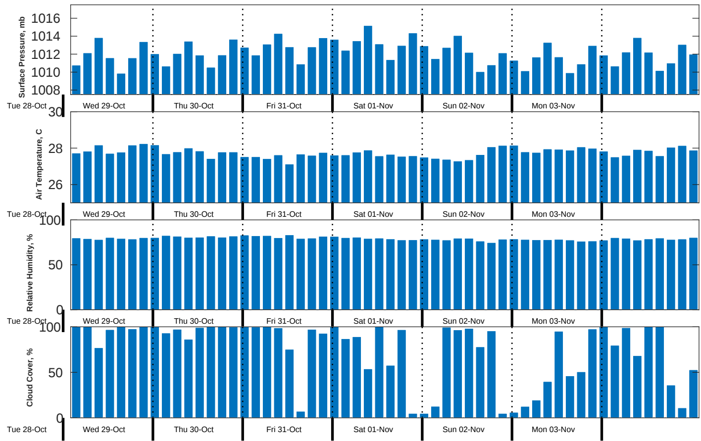
Met Forecast for Proteus from 29-Oct-2025 00:00:00 to 05-Nov-2025 00:00:00
