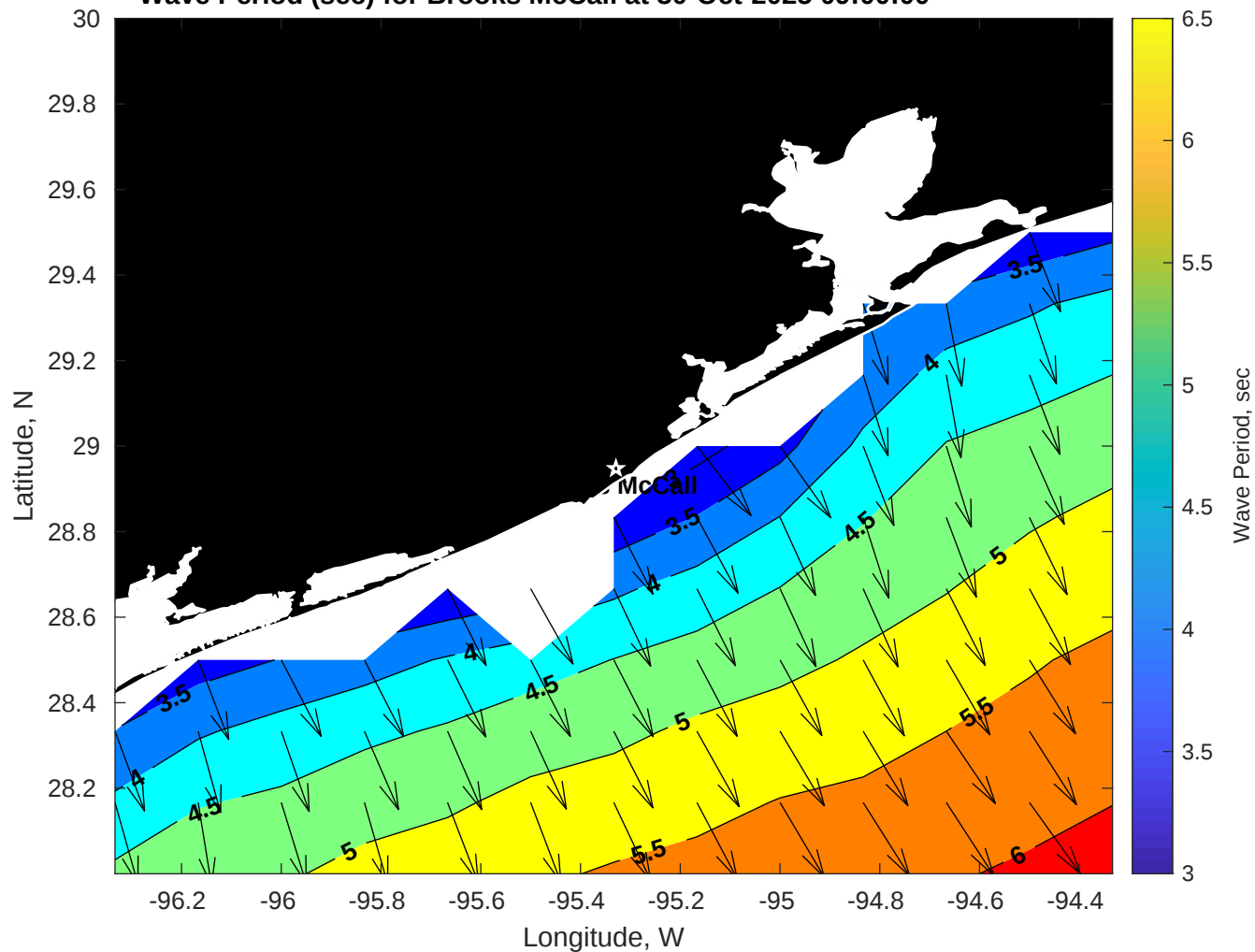
Wave Period (sec) for Brooks McCall at 30-Oct-2025 09:00:00
