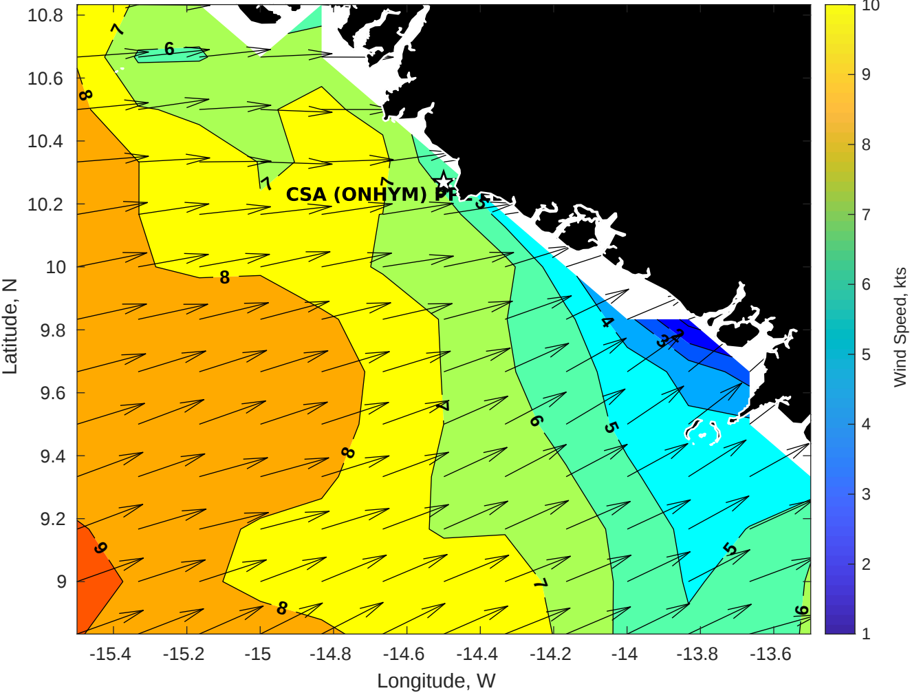
Winds (kts) for CSA (ONHYM) PPL EBS - Guinea at 30-Oct-2025 09:00:00
