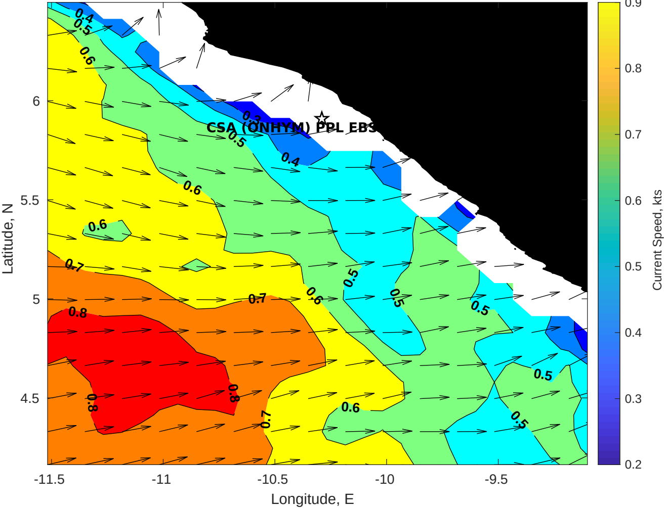
Surface Currents for CSA (ONHYM) PPL EBS - Liberia at 29-Oct-2025 00:00:00
