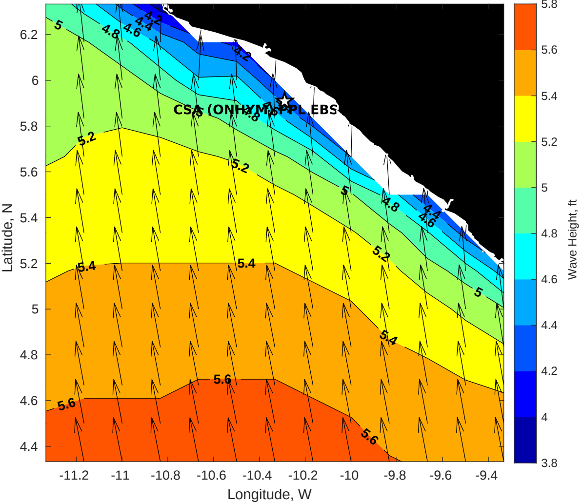
Wave Height (ft) for CSA (ONHYM) PPL EBS - Liberia at 30-Oct-2025 09:00:00
